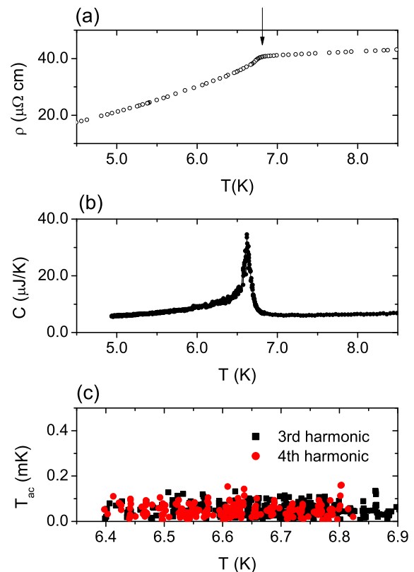
FIG. 1. (a) Temperature dependence of the in-plane electrical resistivity \rho of CeAuSb 2 at ambient pressure. The arrow indicates onset of the antiferromagnetic transition at 6.8 K. (b) Specific heat capacity of CeAuSb 2 . The sharp peak is displaced as a function of temperature relative to the kink in resistivity near T_N . (c) Measurements of 3f and 4f harmonics of T_{ac} while the sample heater is excited at frequency 1f .
