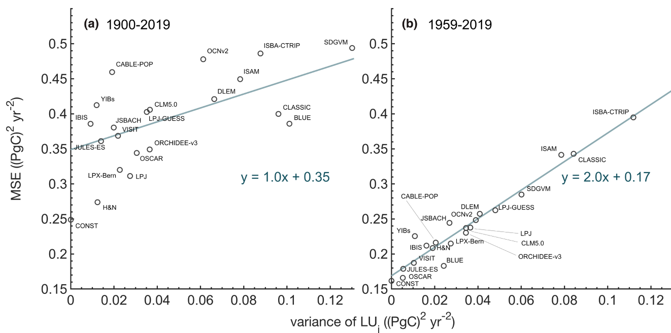
FIGURE 2 Relationship between regression errors in Equation (2) and decadal variability in the land use flux \text{LU}_j used as input, with separate analyses for the 1900–2019 (panel [a]) and 1959–2019 (panel [b]) timeframes. The decadal variability in the land use flux is represented as the variance of the decadal smoothed land use flux over each period after removing a linear trend, and the model errors are shown as the mean annual mean squared error (MSE) over the same period across each land use flux's 10,000-member ensemble. The lines and accompanying equations are a linear least-squares fit to the data excluding CONST. All reported data for the grouped land use fluxes hereafter exclude model runs for the CONST case.
