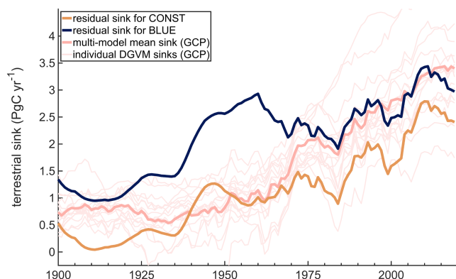
FIGURE 5 Comparisons of terrestrial sink estimates, including sinks inferred as the residual of Equation (1) ( B_{\text{res}} ) assuming different estimates for LU_j where B_{\text{res}} = FF + LU_j - O - AGR , where LU_j is either CONST or BLUE. Thin pink lines represent estimates of individual models of B per Friedlingstein et al. (2020). No adjustment is made to the means of the land use fluxes in this figure. All data have 10-year smoothing applied.
