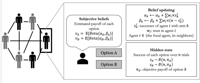
Figure 1: A schematic overview of the agent-based model used in our studies.
