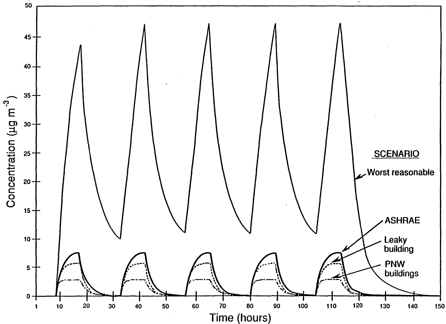
FIGURE 1. Variation in the concentrations of benzene over a period of a work week in an intermediate-size office building for four ventilation-infiltration scenarios.
