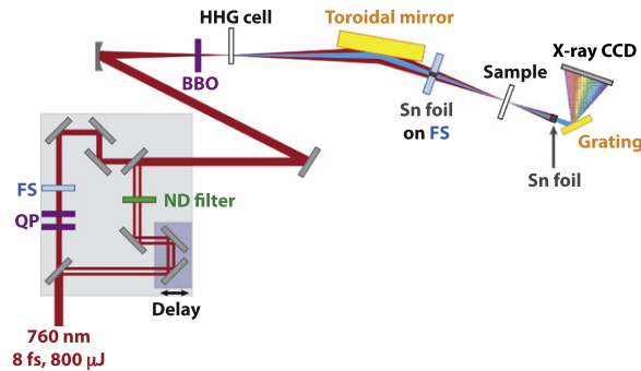
Figure 1. Schematic of experimental set-up. QP =quartz plate, FS =fused silica, ND =neutral density, BBO = \beta -BaB 2 O 4 crystal, HHG =high harmonic generation. QP and BBO are optics used to implement double optical gating.
