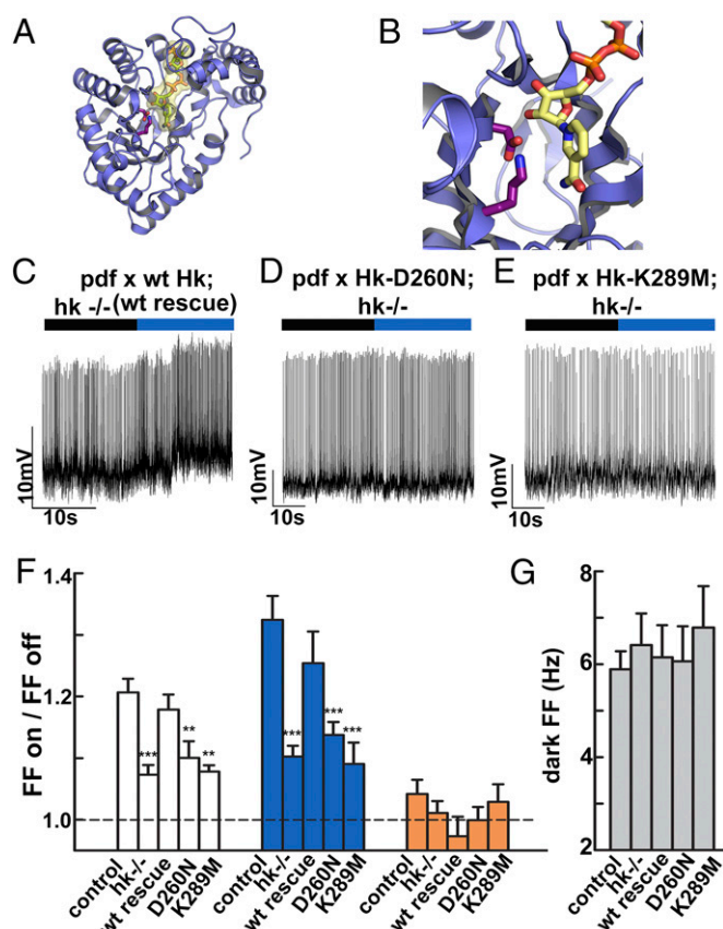
Fig. 3. LNV-directed expression of WT Hk in hk -/- flies functionally rescues the Cry-mediated light response, whereas expression of Hk redox sensor-disabling mutants fail to rescue. (A) Structural model of the Kv \beta subunit (blue) bound to the NADP + cofactor (yellow). (B) Positional model of two key residues for Kv \beta redox sensing (D260 and K289) depicted in stick form in magenta relative to the NADP + cofactor (yellow). (C) WT Hk expressed in LNV neurons in the hk -/- genetic background rescues the I-LNV light response (black bar indicates no light; purple bar indicates 375–450 nm blue light, 0.6 mW/cm 2 ). In contrast, LNV-directed expression of redox-disabled point mutants D260N-Hk (D) and K289M-Hk (E) in hk -/- fail to rescue the I-LNV blue light response. (F) The white light response (firing frequency lights on/lights off, 4 mW/cm 2 ) recorded in I-LNV expressing WT Hk in hk -/- (WT rescue, 1.18 \pm 0.02 , n = 22 ) is indistinguishable from the control response ( 1.21 \pm 0.02 , n = 26 , P = 0.79 ) but is significantly different from hk -/- ( 1.07 \pm 0.02 , n = 16 , P = 0.004 ), showing functional rescue. In contrast, LNV-directed expression of the redox-disabled D260N-Hk mutant in hk -/- ( 1.12 \pm 0.03 , n = 13 ) is significantly different from control ( P = 0.036 ) but not hk -/- ( P = 0.58 ) recordings, indicating failure to rescue. Similarly, the white light response recorded in I-LNV expressing the redox disabled K289M-Hk mutant in hk -/- ( 1.08 \pm 0.01 , n = 12 ) is significantly different from control ( P < 0.001 ) but not null ( P = 0.99 ) recordings. The response to blue light in WT rescue I-LNV recordings ( 1.25 \pm 0.05 , n = 16 ) is not different from control ( P = 0.61 ), but differs from hk -/- ( 1.10 \pm 0.02 , n = 23 , P = 0.038 ); the light response in recordings of I-LNV expressing D260N-Hk is significantly less than from control ( 1.15 \pm 0.02 , n = 15 , P = 0.01 ) and not different from null ( P = 0.88 ); the light response in recordings of I-LNV expressing K289M-Hk in hk -/- ( 1.06 \pm 0.02 , n = 13 ) is significantly less than control ( P < 0.001 ) and not different from null ( P = 0.95 ). In orange light (4 mW/cm 2 , >550 nm), WT rescue ( 0.96 \pm 0.1 , n = 11 ), D260N-Hk ( 1.00 \pm 0.06 , n = 8 ), and K289M-Hk ( 1.03 \pm 0.09 , n = 10 ) are not significantly different from each other, control ( 1.04 \pm 0.11 , n = 23 ), or hk -/- ( 1.01 \pm 0.08 , n = 17 ) recordings ( P > 0.1 in all comparisons). (G) The basal firing frequencies in the dark for control ( 5.89 \text{ Hz} \pm 0.39 , n = 77 ), hk -/- ( 6.41 \text{ Hz} \pm 0.68 , n = 37 ), Hk WT rescue ( 6.15 \text{ Hz} \pm 0.69 , n = 31 ), Hk D260N rescue ( 6.06 \text{ Hz} \pm 0.76 , n = 23 ), and Hk K289M rescue ( 6.79 \text{ Hz} \pm 0.89 , n = 18 ) do not differ ( P = 0.77 , P = 0.941 , P = 0.999 , and P = 0.874 vs. control, respectively). All data values and statistics are presented in detail in Dataset S1 .
