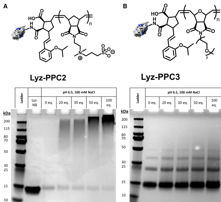
Figure 2. Characterization of Lyz-PPC2 and Lyz-PPC3 by denaturing SDS-PAGE gel
