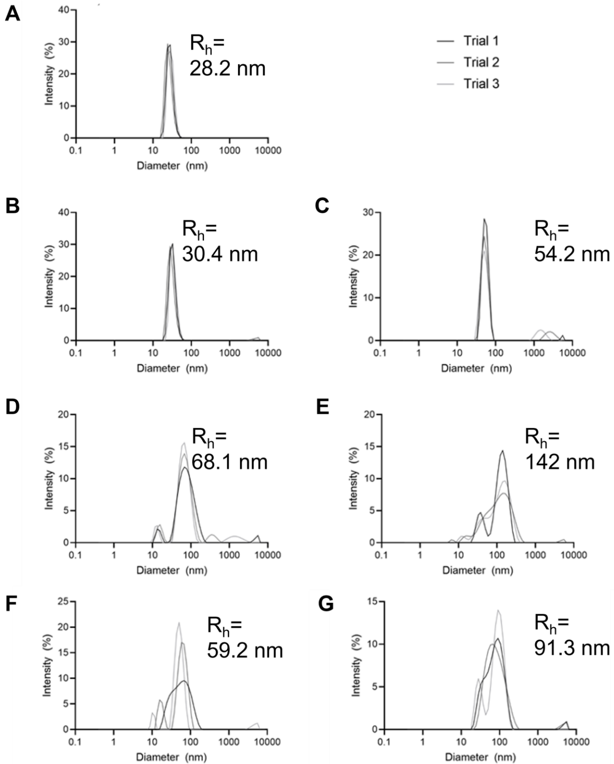
Figure S14. Dynamic light scattering measurements for Q \beta , Q \beta -NB and Q \beta -PPCs.
