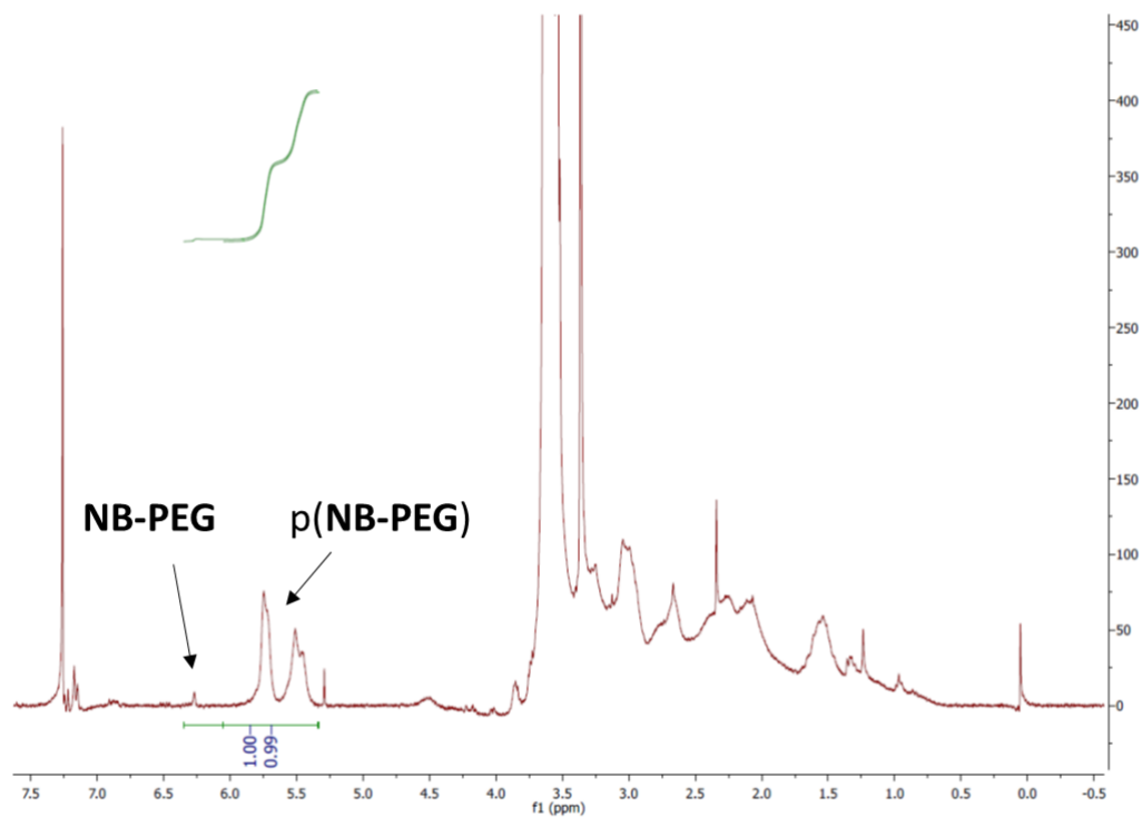
Figure S3. ^1\text{H-NMR} of NB-PEG polymerization in the presence of lysozyme.
