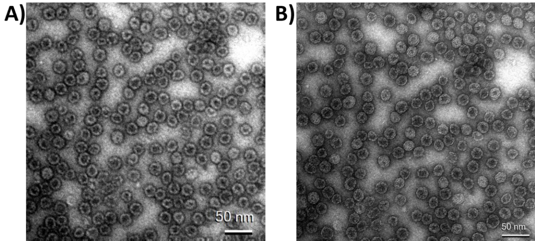
Figure S15. TEM micrographs (scale bar= 50 nm) of Q \beta and Q \beta -NB.
