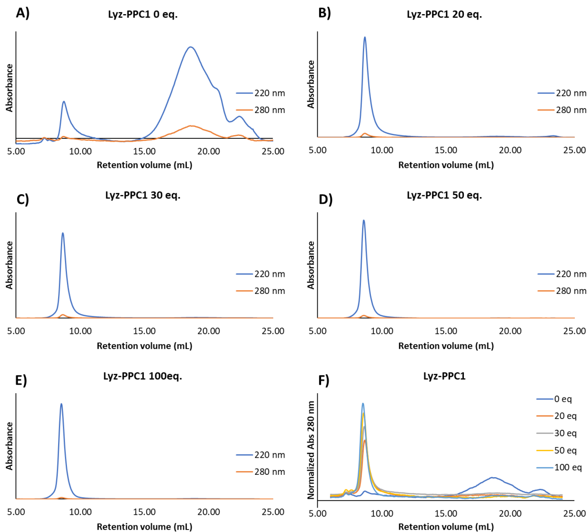
Figure S4. SEC of Lyz-PPC1 synthesized with varying monomer equivalences.
