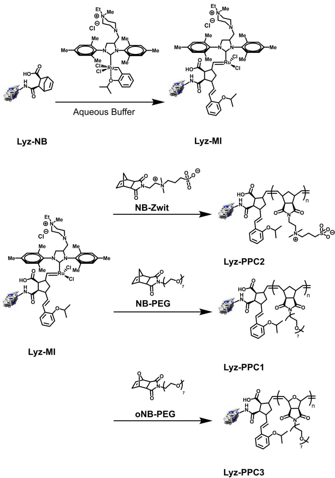
Reaction scheme 1. Synthesis of Lyz-PPC1 , Lyz-PPC2 , and Lyz-PPC3 .
