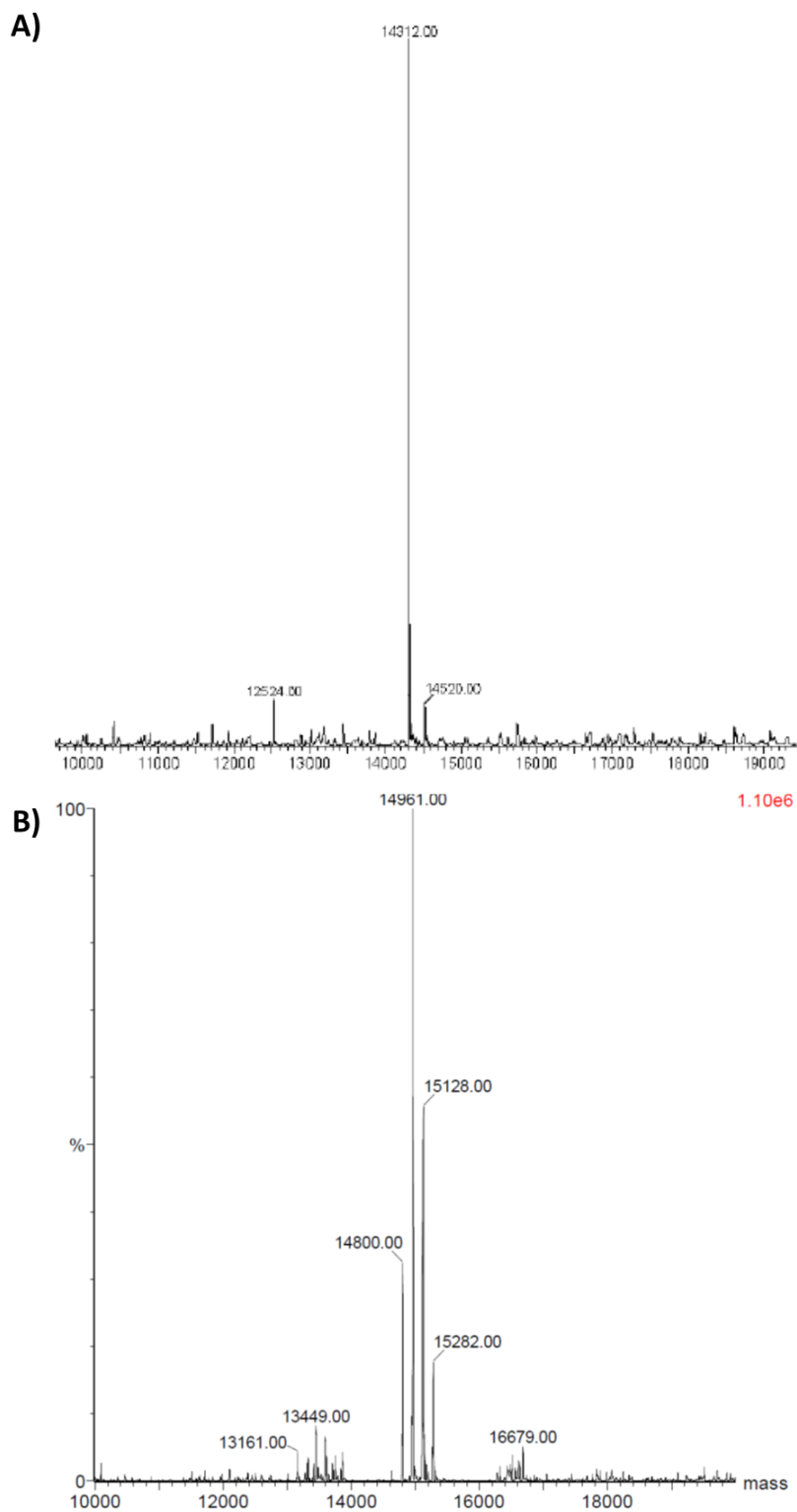
Figure S1. Mass analysis of Lyz and Lyz-NB.
