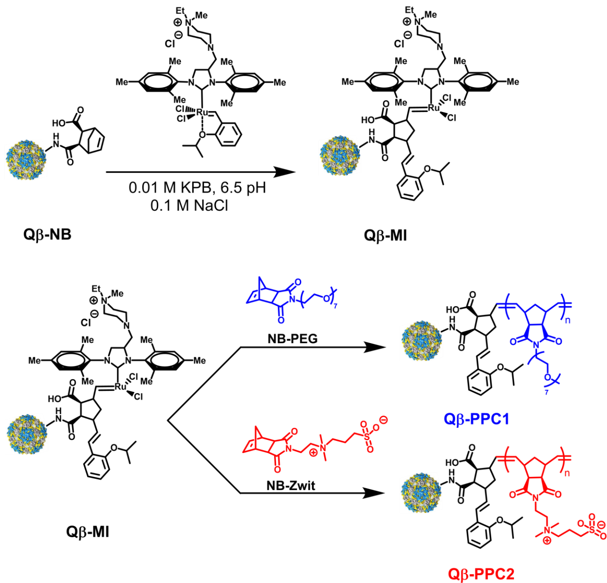
Reaction scheme 3. Synthesis of grafting-from Q \beta -PPCs.
