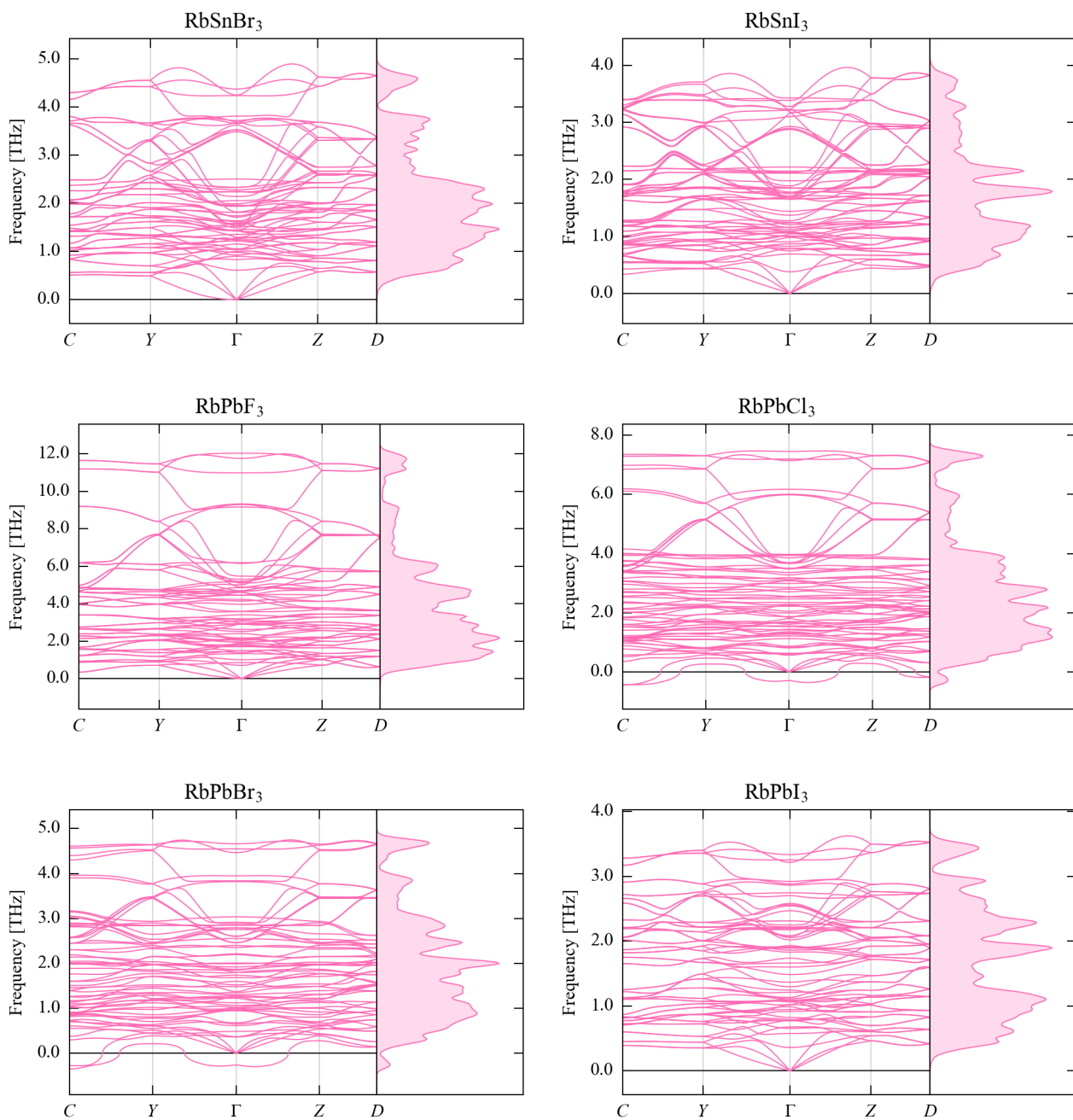
Figure S4: Phonon dispersion and density of states for the monoclinic phase of 24 compounds
