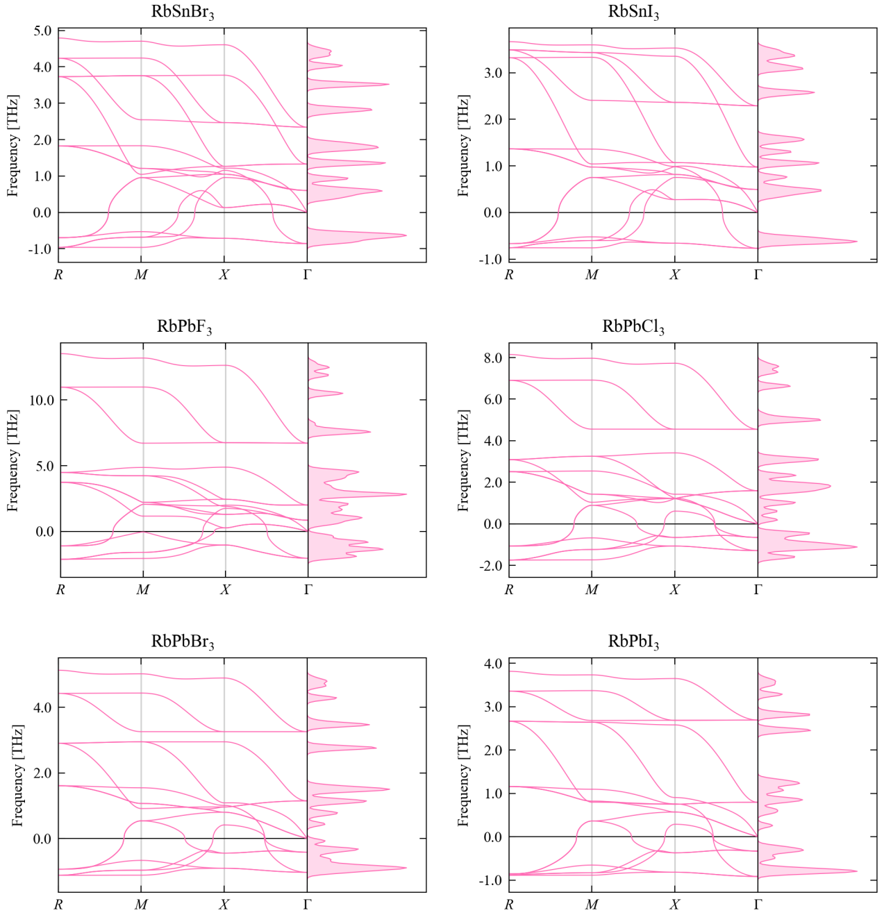
Figure S1: Phonon dispersion and density of states for the cubic phase of 24 compounds
