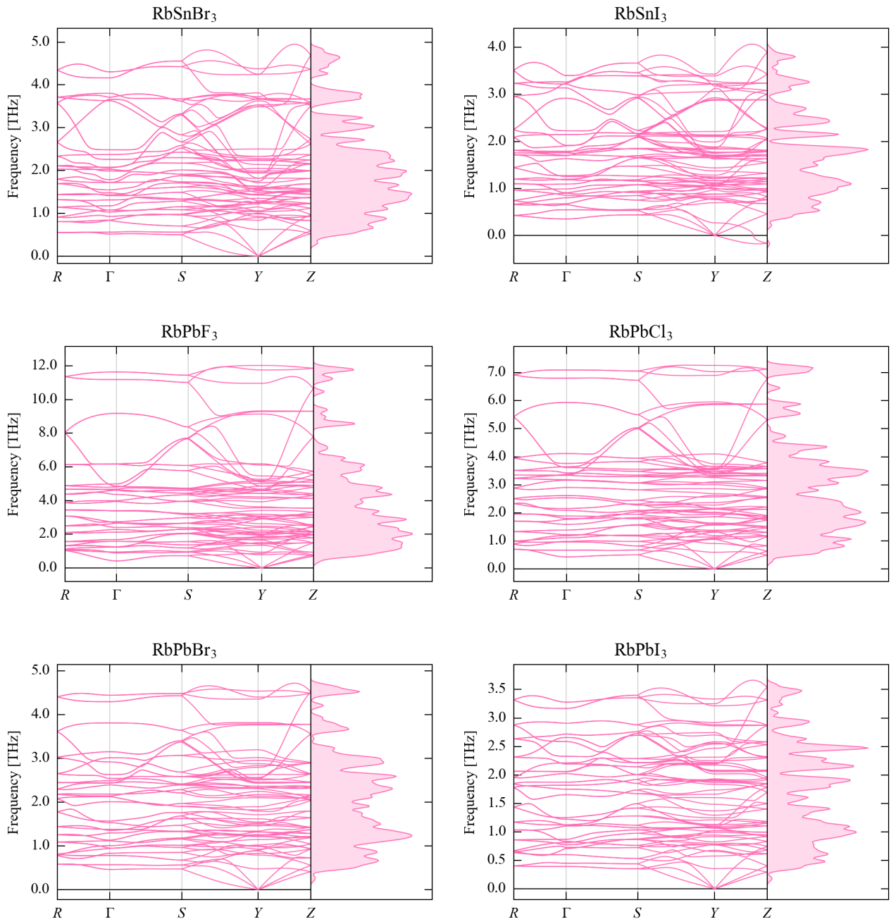
Figure S3: Phonon dispersion and density of states for the orthorhombic phase of 24 compounds
