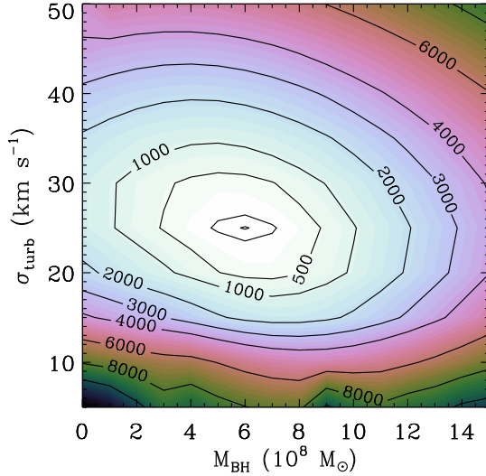
FIG. 8.— Contours of constant \Delta\chi^2 as a function of M_{\text{BH}} and \sigma_{\text{turb}} , for the flat \sigma_{\text{turb}} profile. The minimum \chi^2 value of 11173.4 (for 2540 degrees of freedom) is obtained at M_{\text{BH}} = 6 \times 10^8 M_{\odot} and \sigma_{\text{turb}} = 25 \text{ km s}^{-1} . The two innermost contours correspond to \Delta\chi^2 = 10 and 100. Models were calculated over a grid with increments of 10^8 M_{\odot} and 5 \text{ km s}^{-1} .
