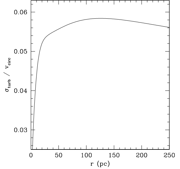
FIG. 16.— Radial profile of \sigma_{\text{turb}}/v_{\text{circ}} for the model with \sigma_{\text{turb}} = 24.7 \text{ km s}^{-1} and M_{\text{BH}} = 6.0 \times 10^8 M_{\odot} .
