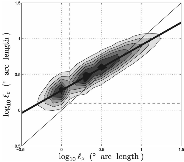
FIG. A1. Contours of binned point density in log–log space of l_c vs l_z , where 5% of the data reside outside the first contour. The thin sloped line indicates l_c = l_z , the bold sloped line is a least-squares linear regression of l_c vs l_z , and the dashed lines bound a box where \log_{10} l_c \geq 0.0986 .
