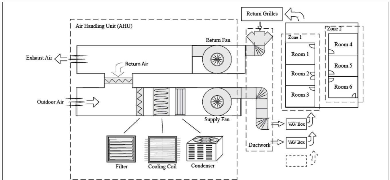
FIGURE 4 | Schema of a variable air volume air handling unit HVAC operational systems.
