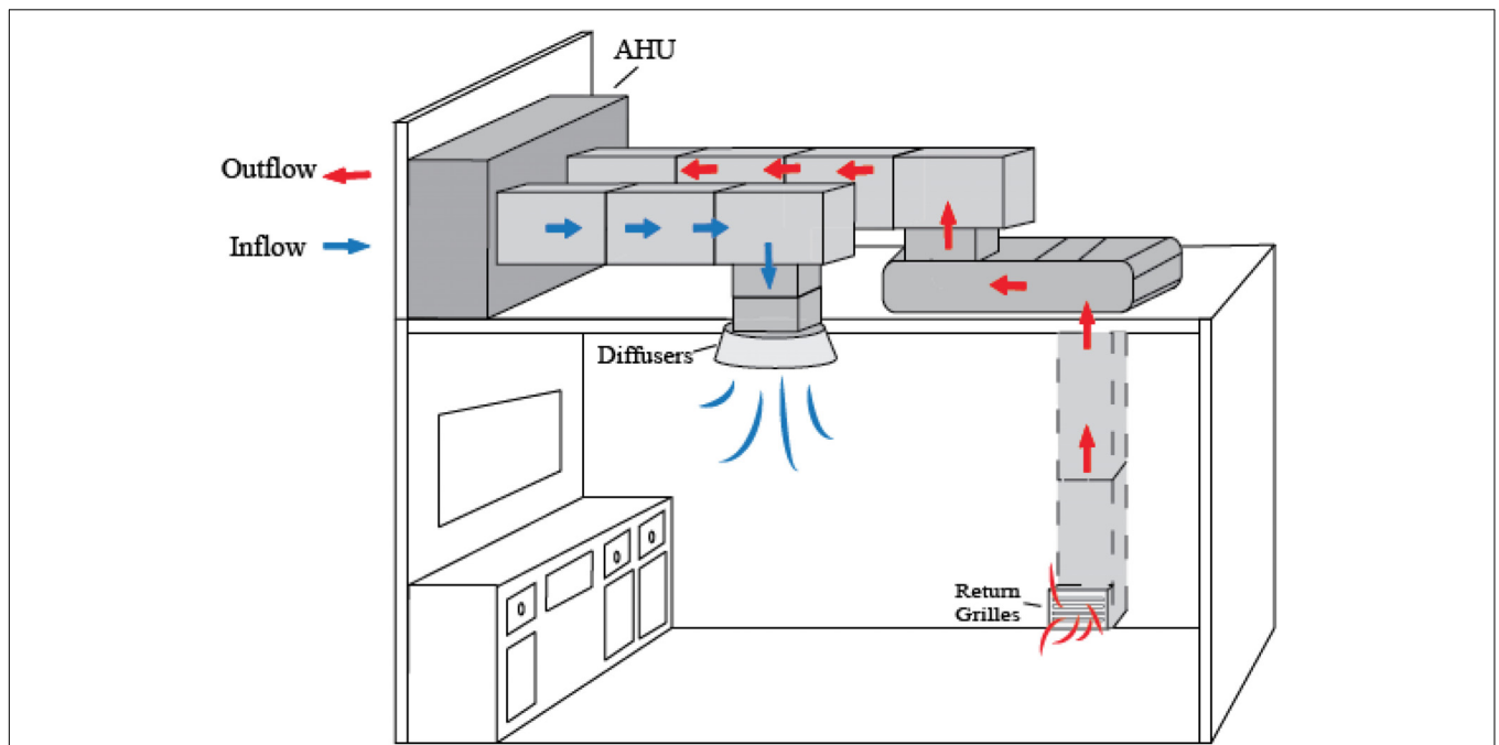
FIGURE 5 | Air circulation via HVAC systems as a means of proper ventilation of space.
