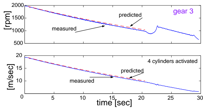
Figure 12: Validation simulations with four activated cylinders show the trajectories of predicted and measured engine speed.
