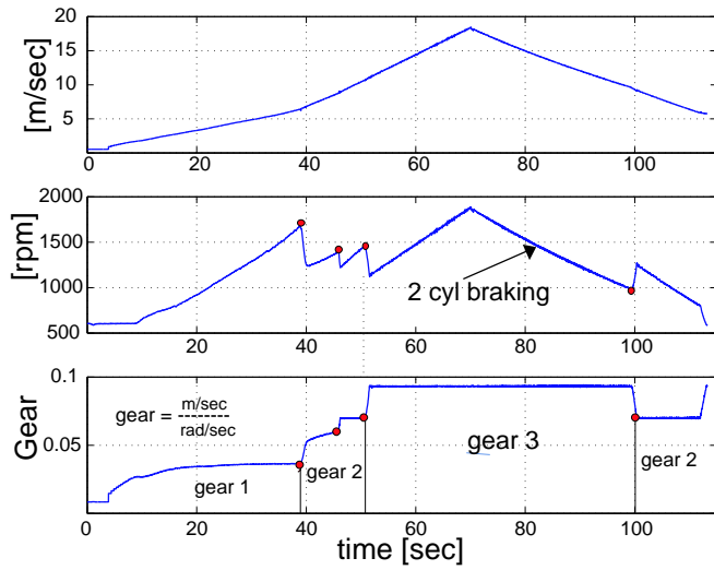
Figure 4: The trajectories of vehicle speed, engine speed and estimated gear ratio.
