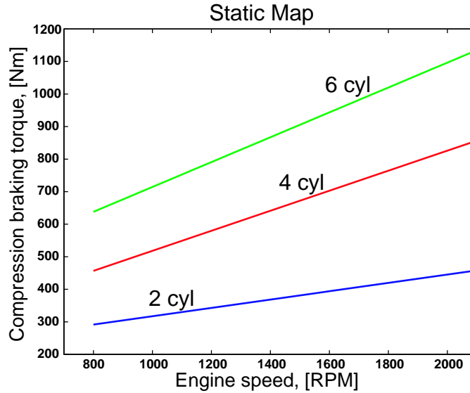
Figure 9: Steady-state engine braking map.
