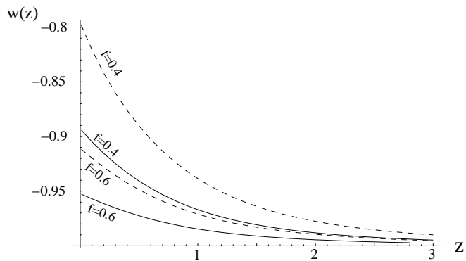
FIG. 2: w(z) for 4 choices of (f/M_{\text{Pl}}, \phi_0/f) . The solid lines are \phi_0/f = 0.6\pi while the dashed lines have \phi_0/f = 0.7\pi . The lines are labeled by their value of f/M_{\text{Pl}} .
