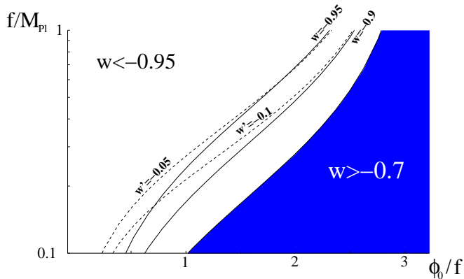
FIG. 1: Contours for w and w' .
