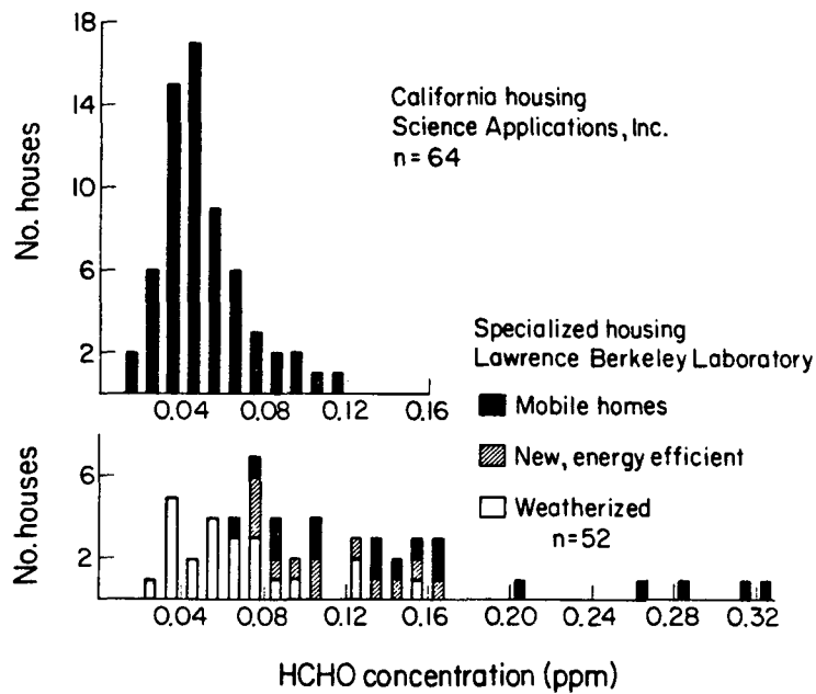
Figure 4-4. Residential formaldehyde concentrations
