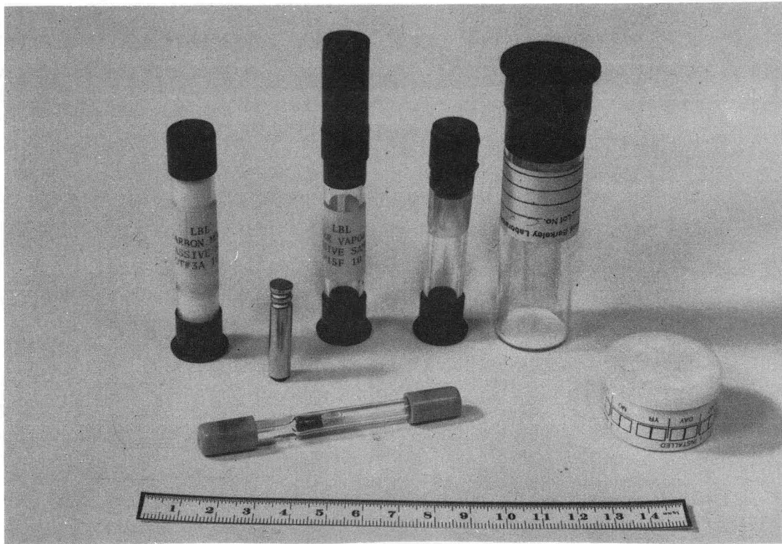
Figure 6-3. Passive samplers--left to right (back): Carbon monoxide, infiltration source, water vapor, nitrogen dioxide, formaldehyde; (front): infiltration (sampler), radon.
