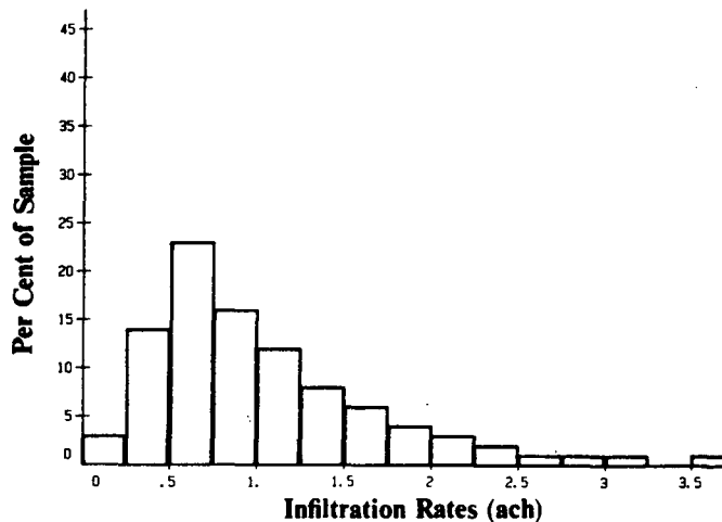
Figure 2-3. Infiltration rates in U.S. houses
