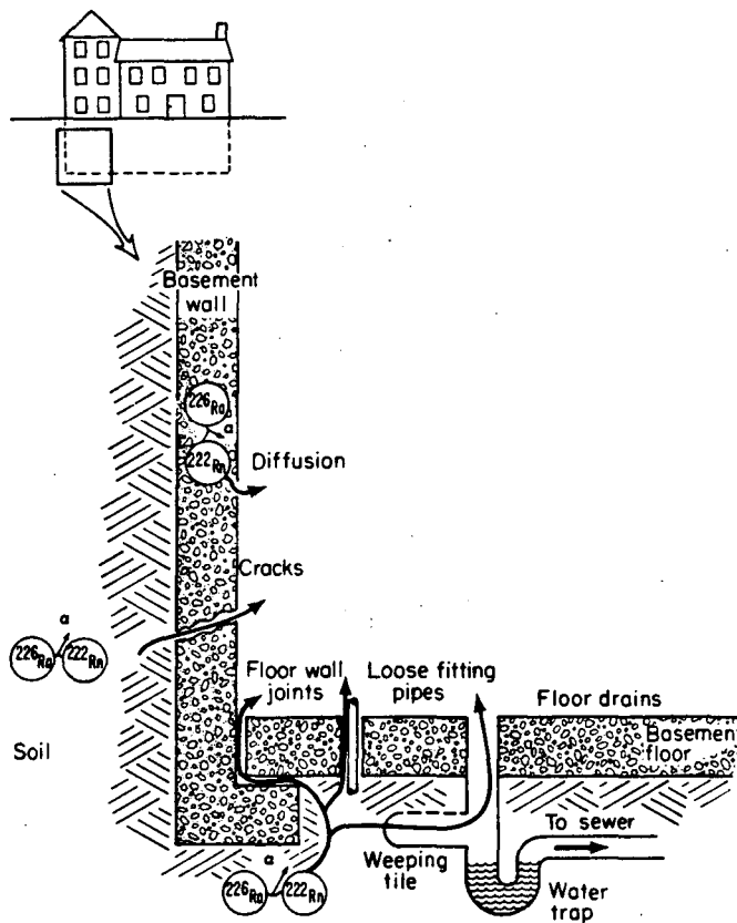
Figure 4-2. Primary pathways for radon entry into buildings
