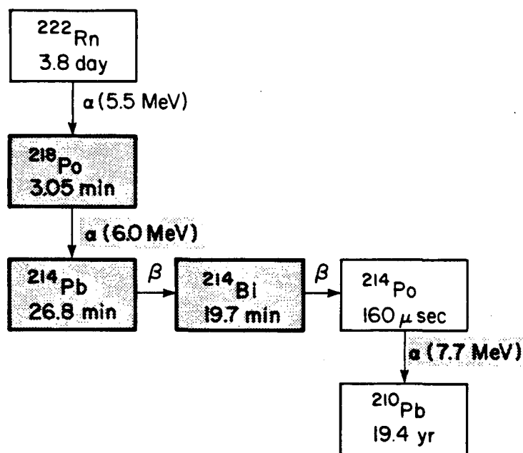
Figure 4-1. Radon decay chain
