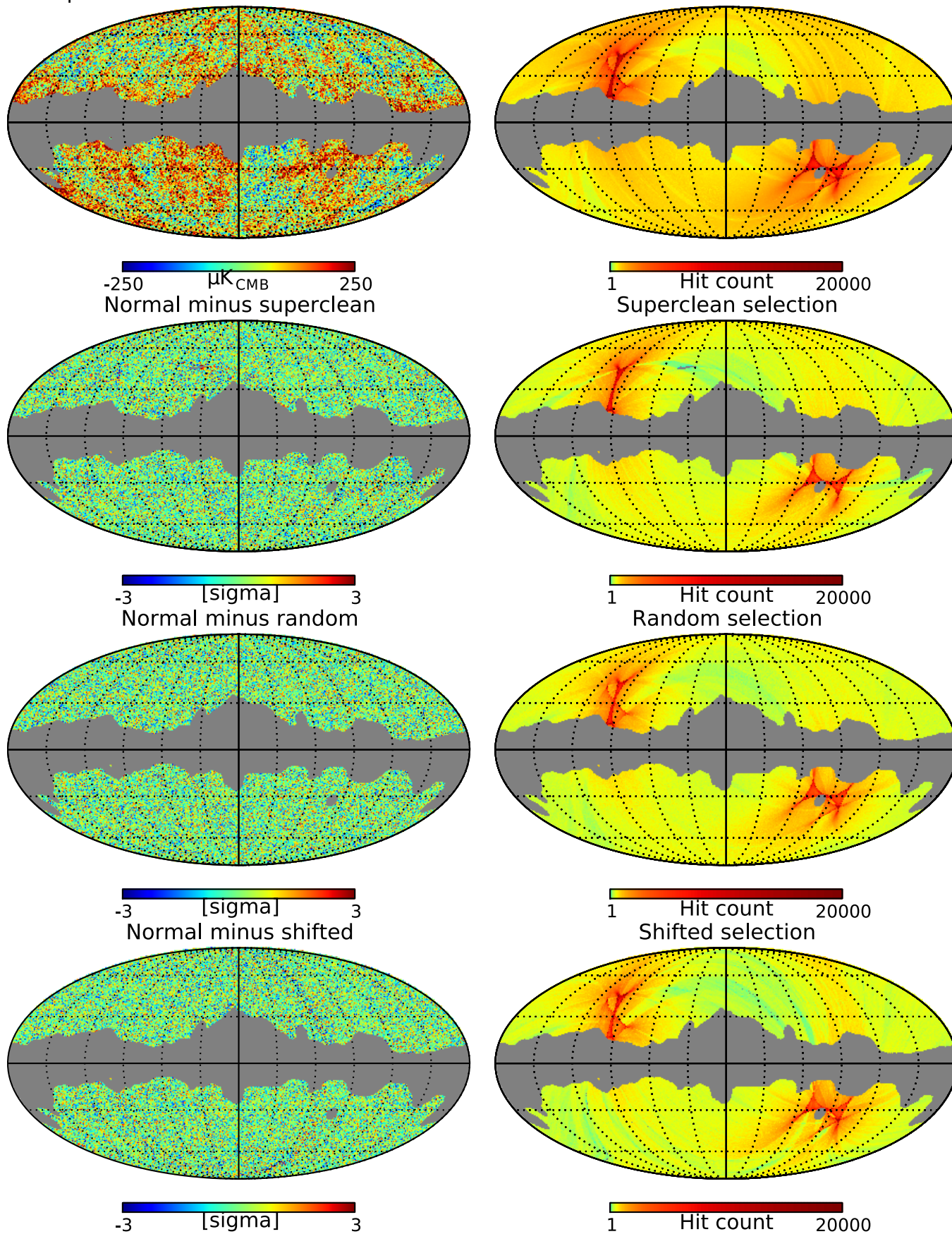
Fig. B.2. Top panels: 143 GHz intensity (left) and corresponding hit-count map (right). Lower panels: difference (left) between a given selection and normal maps, whitened with the noise calculated from the corresponding hit-count map (right), in units of the standard deviation. For the severe selection, striping of the hit numbers is more visible.
