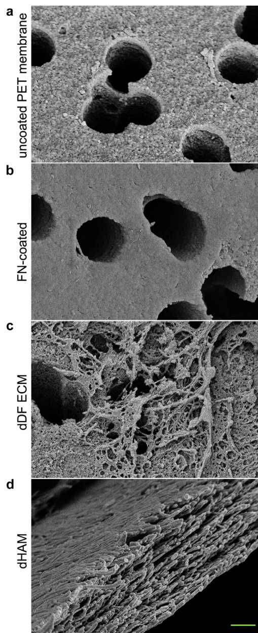
Figure 1. SEM images of epidermal basement membrane substitutes used for bioengineering of HEEs. (a) Uncoated PET membrane of Transwell inserts. (b) FN-coated PET membrane, (c) dDF ECM, and (d) dHAM used as a substrate for growing HEEs. Bar = 200 nm. dDF ECM, decellularized dermal fibroblast-produced and –assembled extracellular matrix; dHAM, dry human amniotic membrane; FN, fibronectin; HEE, human epidermal equivalent; PET, polyethylene terephthalate; SEM, scanning electron microscopy.
