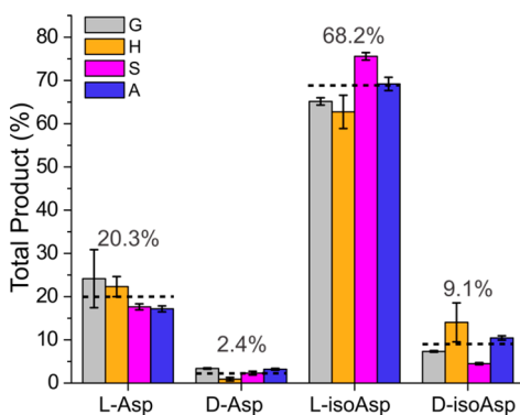
Figure 3. Deamidation products at 37 °C in 50 mM Tris at pH 7.8. Averages are indicated with dashed lines.
