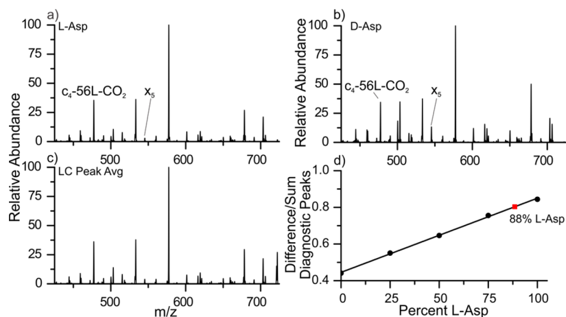
Figure 2. (a,b) Standards of the L-Asp and D-Asp isomers of 4IB-VKLDGS are distinguished by diagnostic fragment peaks. (c) The average fragmentation abundance for the LC peak that contains both isomers. (d) A calibration curve generated from purified standards reveals the LC peak contains 88% L-Asp (red square).
