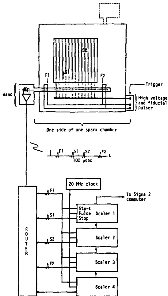
FIG. 9. Schematic of the spark digitizing electronics. F1 and F2 are pulses from the fiducial wires, and S1 and S2 are pulses from sparks.
