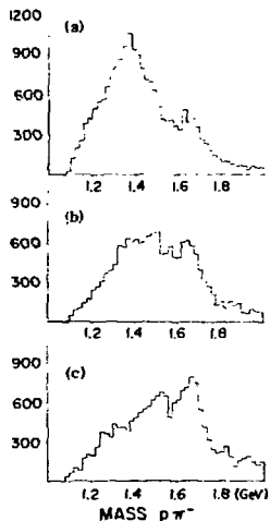
Mass spectra of p\pi^- pairs in hydrogen, integrated over a 50–300 GeV/c neutron momentum band, displayed as a function of t . (a), (b), and (c) correspond to |t| bands of 0.02–0.08, 0.08–0.20, and 0.20–1.00 GeV 2 , respectively.
