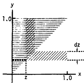
FIG. 39. Integration regions in the domain of H(x,y) for P(H_F) and \ell(z) .
