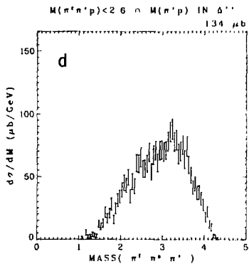
FIG. 17. A_1 and A_3 enhancements are visible in the scattergram of events with M(N^*) < 3.4 GeV. We illustrate suppression of the A's by b) the cut M(N^*) < 2.6 GeV, c) this cut combined with M(\pi^+ \pi^+) > 1.45 GeV, and d) this cut combined with selection of \Delta^{++} by the cut 1.15 < M(\pi^+ p) < 1.32 GeV.
