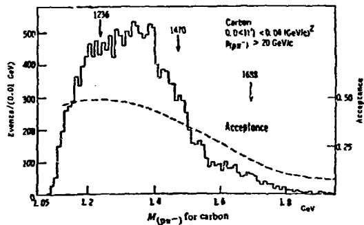
Coherent production cross section versus M_{(p\pi^-)}
