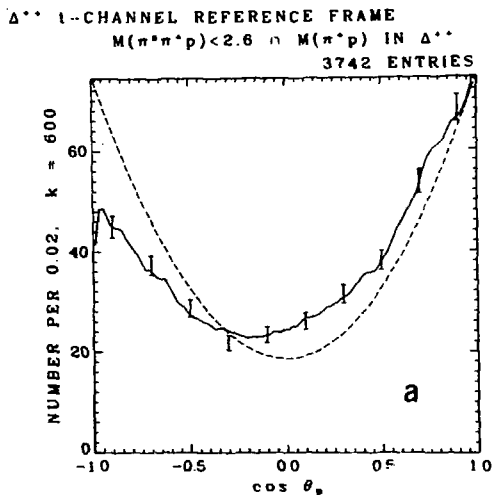
FIG. 25. a) Polar and b) azimuthal distributions for the \Delta^{++} decay in the \Delta^{++} t-channel reference frame (Fig. 8a). Included are all events with 1.15 < M(\pi^+p) < 1.32 GeV. The dashed curve in a) is the function 1+3 \cos^2 \theta_p normalized to the number of events. The data would take this shape if the \pi^+p system were pure J^P=3/2^+ and if J_z were a mixture of +1/2 and -1/2 . Under these same conditions the \phi_p distribution would be uniform.
