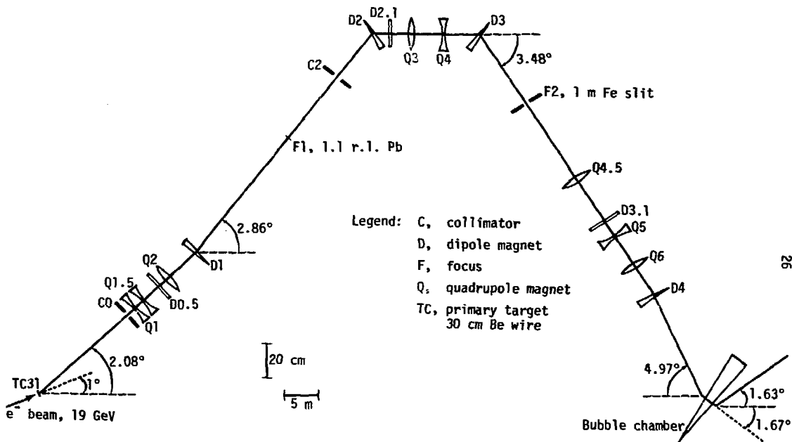
FIG. 7. Elevation view of the secondary beam line. The function of this beam line was to form a 14 GeV/c \pi^- beam and transport it to the bubble chamber. All major bends were in the vertical plane. The field strengths in the horizontal trim magnets D0.5, D2.1, and D3.1 were nominally zero.
