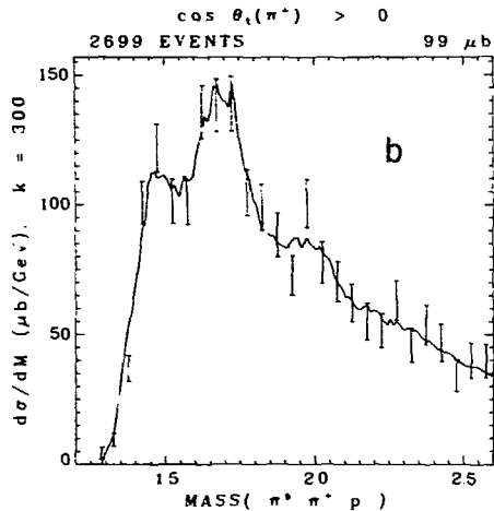
FIG. 30. Distributions of the N^* mass after cuts on a) \cos \theta_s(\pi^+) and b) \cos \theta_t(\pi^+) . These samples are free of A , \rho^0 , and f background and are suitable for tests of helicity conservation. Comparison with Fig. 22 may be helpful.
