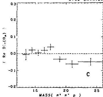
FIG. 26. Moments of the \Delta^{++} decay distribution in the \Delta^{++} t-channel frame (defined in Fig. 8a). The abscissa is M(N^*) in a), b), and c), M(\pi^+p) in d) and e), and -t(p \rightarrow \Delta^{++}) in f) and g).
