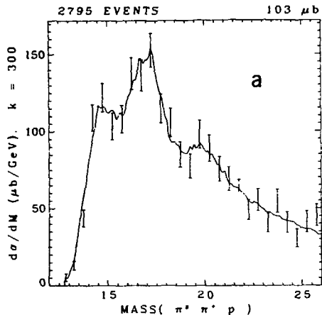
FIG. 30. Distributions of the N^* mass after cuts on a) \cos \theta_s(\pi^+) and b) \cos \theta_t(\pi^+) . These samples are free of A , \rho^0 , and f background and are suitable for tests of helicity conservation. Comparison with Fig. 22 may be helpful.
