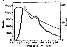
Uncorrected p\pi^+\pi^- mass spectrum for p+C \rightarrow p\pi^+\pi^-+C at 22.5 GeV with -t' < 0.04 (GeV/c) 2 . Geometrical acceptance of the spectrometer vs mass is superimposed.
