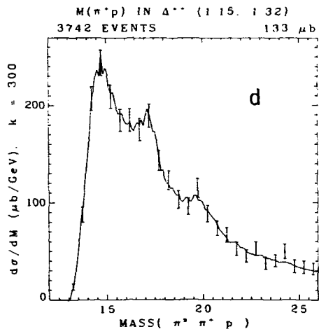
FIG. 22. a) Distribution of the N^* mass after a cut which removes the A , \rho^0 , and f in the \pi^f \pi^s \pi^+ and \pi^f \pi^+ systems. We discuss the dotted and dashed curves in Section IV.8 b,c) The distribution after additional cuts to select \Delta^{++} and \Delta^0 . d) With only the \Delta^{++} cut. This sample is also free of A , \rho^0 , and f .
