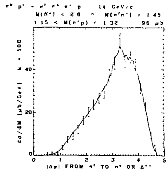
FIG. 20b. Rapidity difference of \pi^f and the closer of \pi^S and \Delta^{++} .
