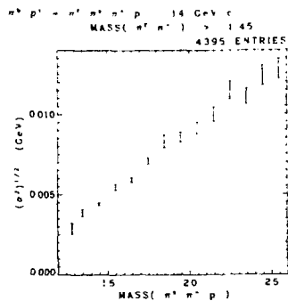
FIG. 19. Mass resolution for the \pi^S \pi^+ p system (r.m.s. of the errors calculated by SQUAW). The resolution for the two-body masses is similar.
