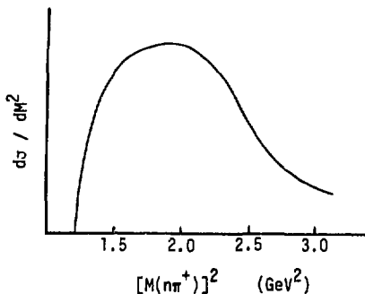
FIG. 2. d\sigma / dM^2 for a Deck model.
