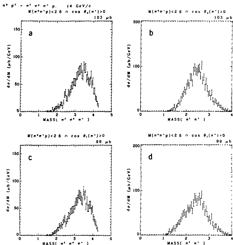
FIG. 29. The cuts on \cos \theta_S(\pi^+) , a) and b), and on \cos \theta_t(\pi^+) , c) and d), eliminate A, \rho^0 , and f signals in meson systems which include the \pi^f . These cuts are suitable for use with tests of helicity conservation. Comparison with Figs. 17 and 18 may be helpful.
