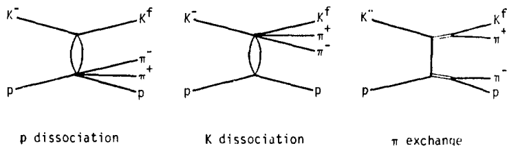
FIG. 15. Diagrams contributing to reaction (3.5b).
