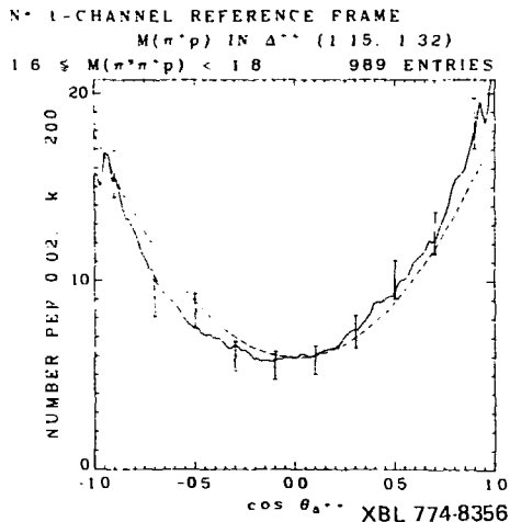
FIG. 28. The polar distribution of the decay N^* \rightarrow \pi^S \Delta^{++} in the t-channel frame for events in the 1.72 GeV enhancement. The dashed curve is the function 1+2 \cos^2 \theta_{\Delta^{++}} normalized to the number of events. A J^P=5/2^+ N^* would generate this shape under some circumstances (see text). We argue that the good agreement here is quite likely fortuitous.
