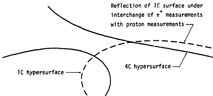
FIG. 38. Schematic of 4C and 1C hypersurfaces.
