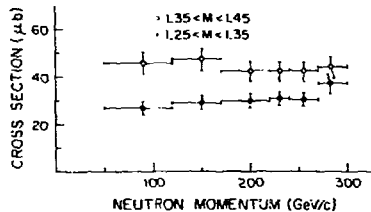
Energy dependence of the cross section for two low-mass intervals. Data are shown integrated over 0.02 < |t| < 1.0 GeV 2 . The absolute normalization is uncertain by about \pm 2\% .
