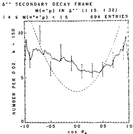
FIG. 27. The polar distribution of the \Delta^{++} decay in the \Delta^{++} secondary decay frame (Fig. 8b) for events near 1.47 GeV. The dashed curve is the function 1+3 \cos^2 \theta_p normalized to the number of events. This shape would result from the second decay of the sequence N^*(1470) \rightarrow \pi^- \Delta^{++} \rightarrow \pi^- \pi^+ p .
