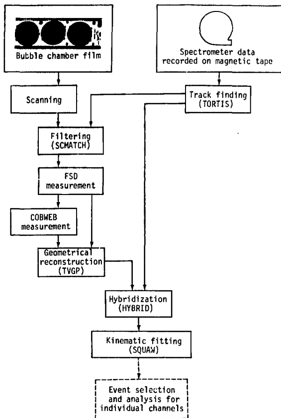
FIG. 11. Preparation of the data for analysis: major processes and the flow of information. FSD and COBWEB designate measuring engines. TORTIS, SCMATCH, TVGP, HYBRID, and SQUAW are computer codes.
