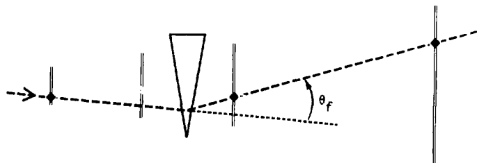
FIG. 37. A triplet of sparks at stations 1, 3, and 4 determines a trajectory through the spectrometer.
