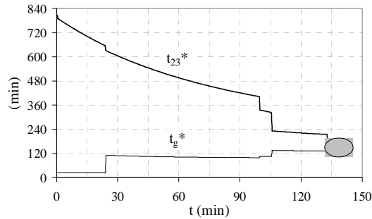
Figure B2-2. Estimates of the time to voltage collapse for #23 and the next PV-PQ transition with respect to t=0 in the IEEE 39-bus system with 75% PQ and 25% Z load.
