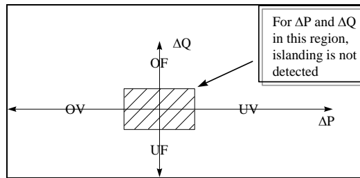
Figure B-5. A nondetection zone (NDZ) defined within the “power mismatch space” Error! Reference source not found.
