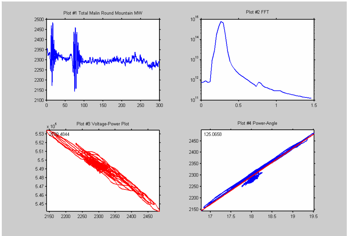
Figure A-10. Analysis of properties as measured on the California Oregon Intertie at Malin Substation: (a) Malin – Round Mt. MW; (b) frequency spectrum of MW flow; (c) slope of P-V curve using Malin Voltage; (c) slope of power-angle curve using John Day to Malin phase angle.
