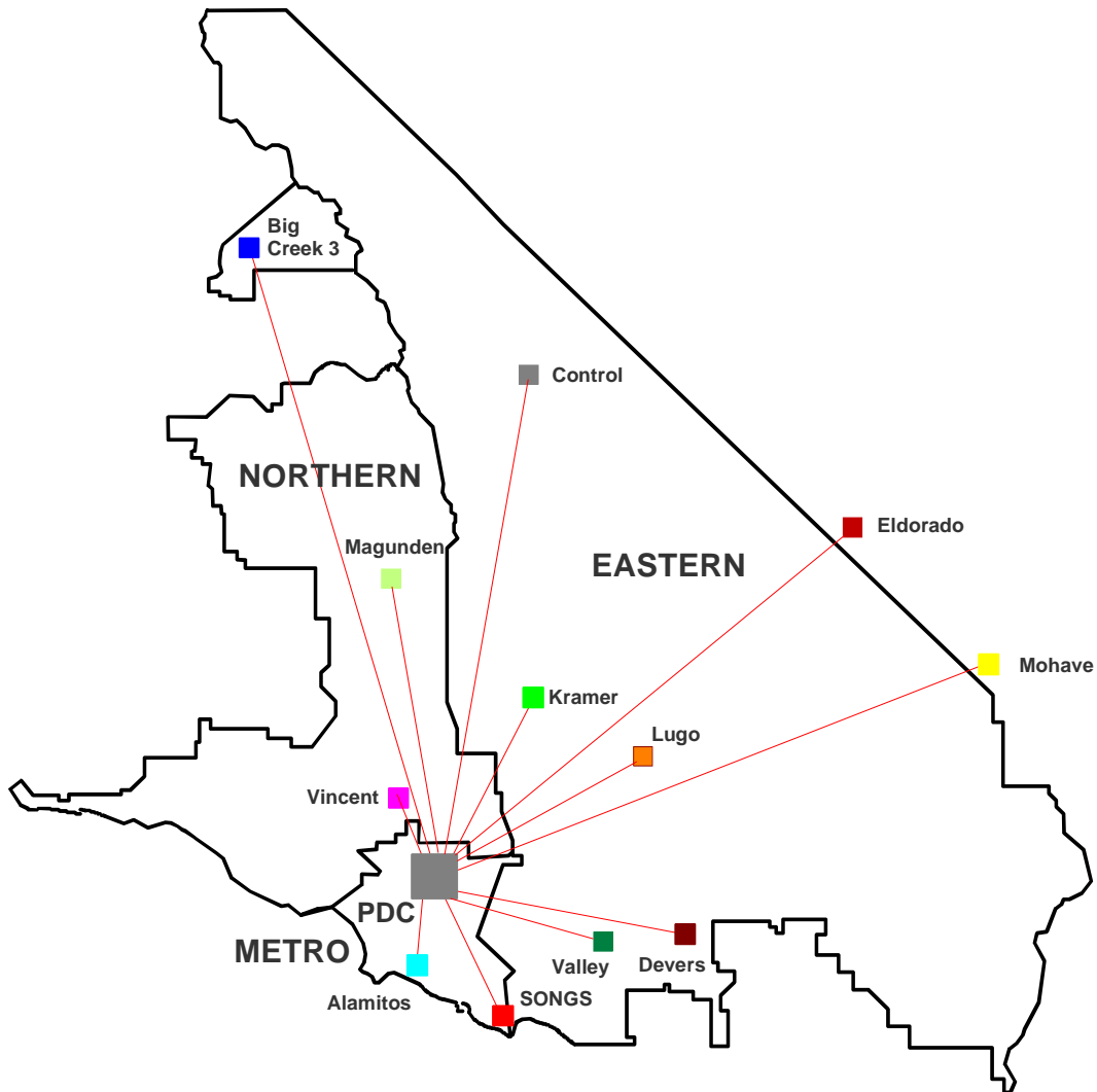
Figure A-12. Phasor Measurement Units installed in SCE
