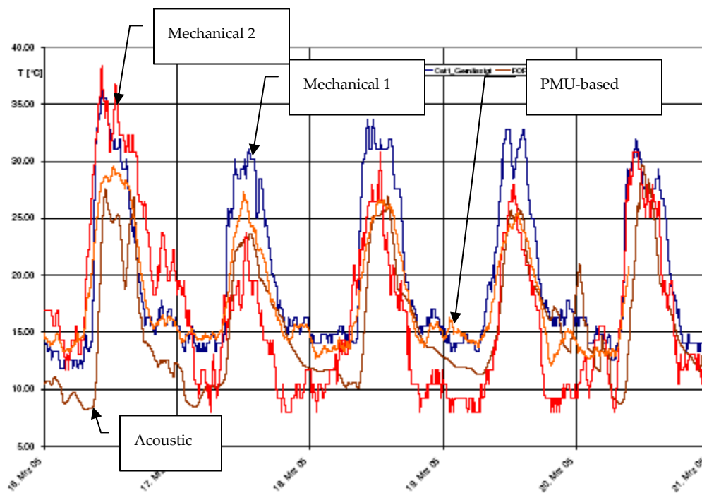
Figure B-6. Comparison of different thermal measuring systems over five days Error! Reference source not found.
