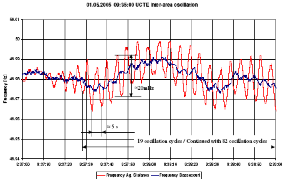
Figure B-3. Oscillations observed by two PMUs on the European grid Error! Reference source not found.
