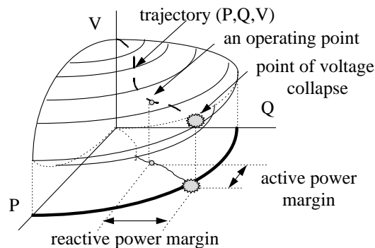
Figure B2-1. Depiction of the process of coalescing of the stable and unstable power system equilibria through slow load variations leading to a voltage collapse. VPQ curve representing the trajectory of the load voltage V of a 2-bus system model when active ( P ) and reactive ( Q ) power of the load change arbitrarily
