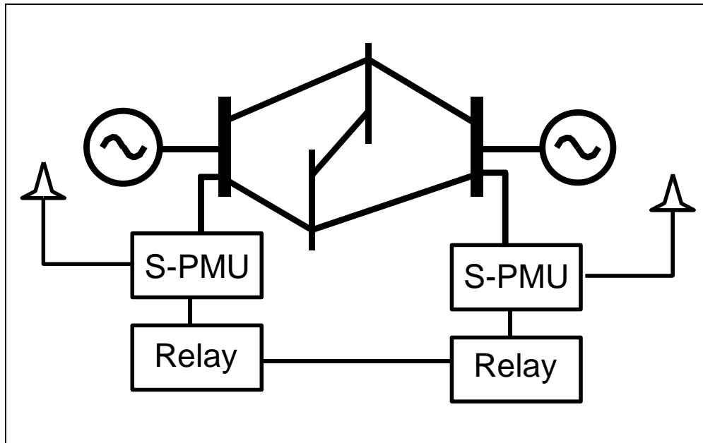
Figure B-7. Out-of-step protection with PMUs.
