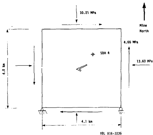
Fig. 10. Loading and boundary conditions of the 176 m level horizontal section.
