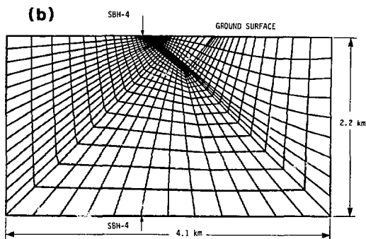
Fig. 18(b). Finite element mesh for the vertical section with double rectangular opening. Rock elements are put back between the openings.
