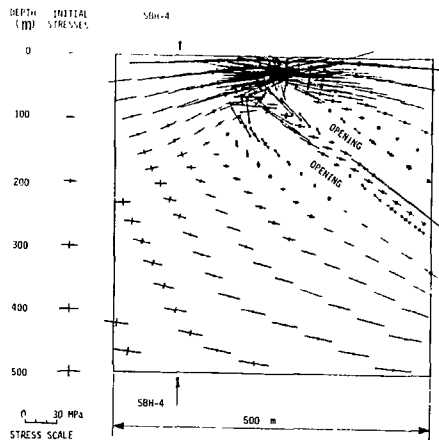
Fig. 19(b). Principal stress distribution in the vertical section with double rectangular openings. Depth and magnitude of initial stresses are shown on left. Arrows denote tension.
