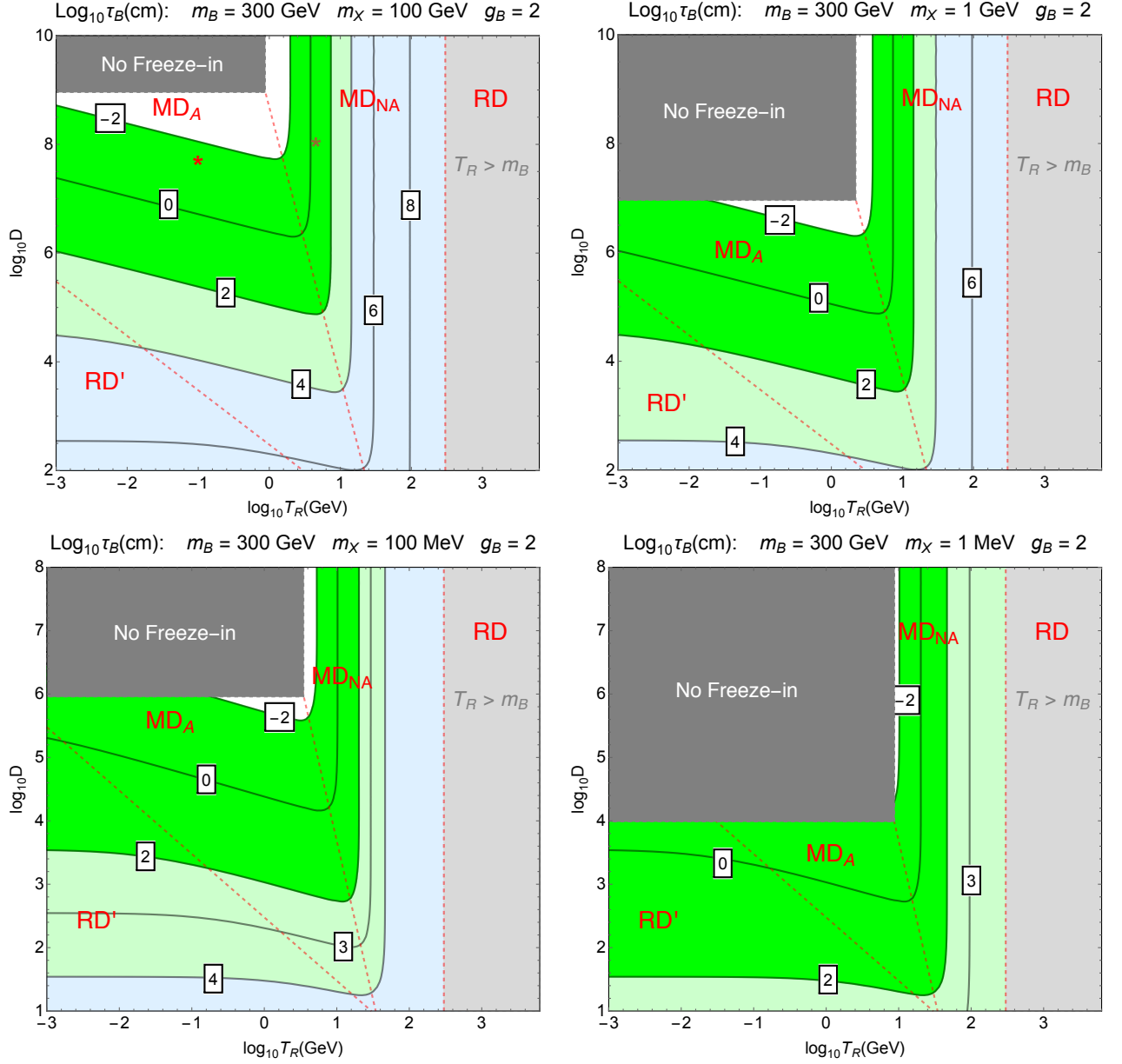
Fig. 28: Contours of the parent particle lifetime \tau_B (in cm) that give the observed DM abundance via FI, assuming that some mechanism dumps entropy into the SM sector at temperature T_R to reduce the DM abundance by dilution factor D . We fix m_B = 300 GeV and in each panel we consider different values of m_X . The upper-left gray region does not give FI, as X thermalizes. The three dashed red lines separate four regions where FI occurs during (left to right) RD', MD A , MD NA , and RD eras. Displaced collider signals occur in almost the entire parameter space. Light green and blue shaded regions in particular are prime targets for MATHUSLA. (This figure is taken from [317], which studied the benchmarks marked by the red and brown stars.)
