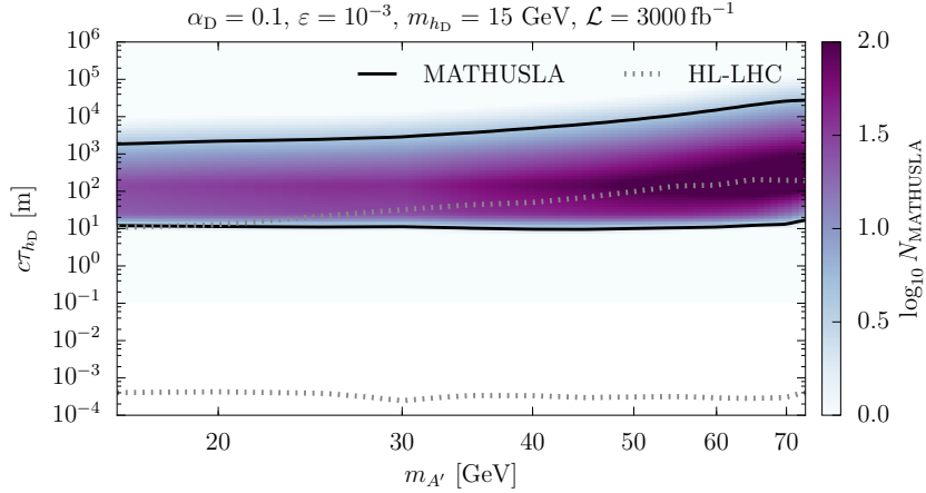
Fig. 64: Sensitivity of MATHUSLA to the dark Higgs-strahlung process is shown in bold solid lines for the case where \alpha_D = 0.1 , \varepsilon = 10^{-3} , and m_{h_D} = 15 GeV with varying m_{A'} mass. The colormap shows the approximate event yield and demonstrates that MATHUSLA has sensitivity to proper lifetimes in the 10 - 10^4 m range. By comparison, the sensitivity of ATLAS and CMS is shown by the region within the gray dotted lines; their reach is optimal for lower lifetimes. This estimate assumes the 200m \times 200m \times 20m benchmark geometry of Fig. 1.
