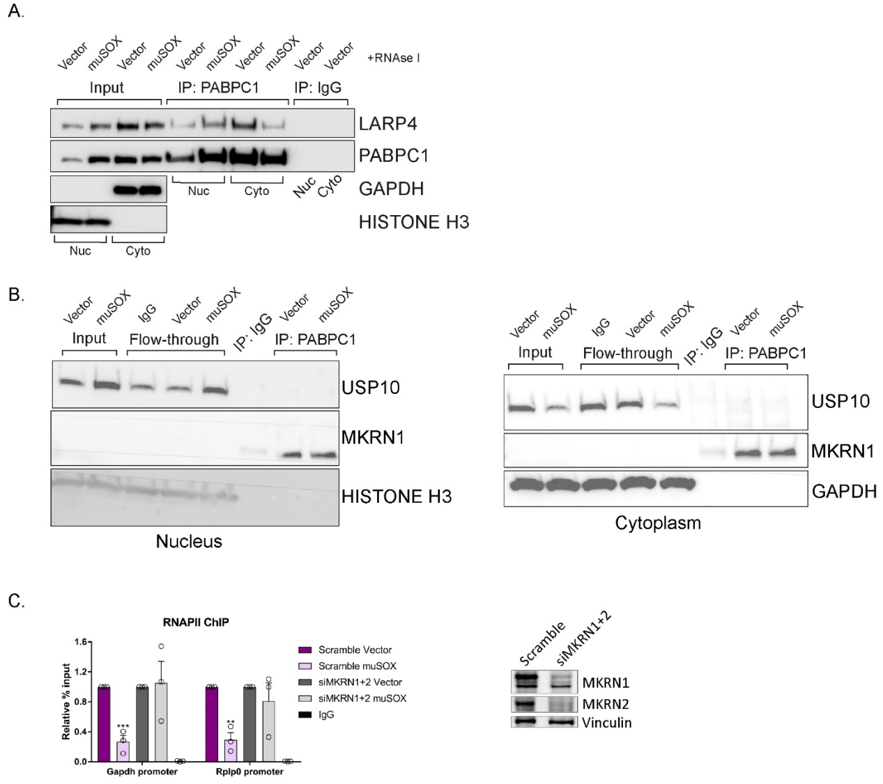
Figure 3.4. Depletion of the E3 ubiquitin ligases MKRN1 and MKRN2 restores RNAPII promoter occupancy during muSOX expression. (A) Western blots from PABPC1 or control IgG co-immunoprecipitations (Co-IPs) from nuclear and cytoplasmic fractions of either vector transfected, or muSOX transfected HEK293Ts. GAPDH and HISTONE H3 in the input samples serve as fractionation controls. (B) Western blots from PABPC1 or control IgG co-immunoprecipitations (Co-IPs) from nuclear (left panel) and cytoplasmic (right panel) fractions of either vector transfected, or muSOX transfected HEK293Ts. GAPDH and HISTONE H3 in the input samples serve as fractionation controls. (C) HEK293T cells treated with siRNAs targeting MKRN1 and MKRN2, or non-targeting scramble siRNAs were subsequently transfected with either empty vector or muSOX, then subjected to chromatin immunoprecipitation (ChIP) using antibodies to RNAPII or IgG. Purified chromatin was quantified by RT-qPCR. Western blots showing protein levels after siRNA depletion are shown, along with a loading control. Graph displays individual biological replicates as dots, with the mean and SEM. Statistical significance was determined using Student's t test * p < 0.05 ** p < 0.005 *** p < 0.0005 .
