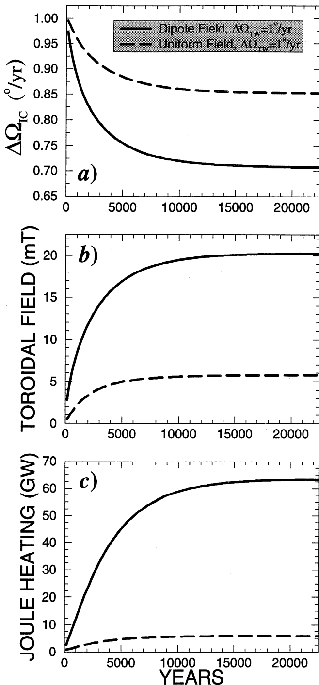
Figure 5. Time series plots of (a) the anomalous rotation of the inner core \Delta\Omega_{IC} , (b) the maximum induced toroidal magnetic field B_{T\max} , and (c) the Joule heating in the core resulting from a 1^\circ/\text{yr} thermal wind acting on a current-carrying dipole and a uniform poloidal magnetic field. The calculations were made using a 120 \times 120 grid for 25,000 simulated years. Steady state is reached after approximately 20,000 years.
