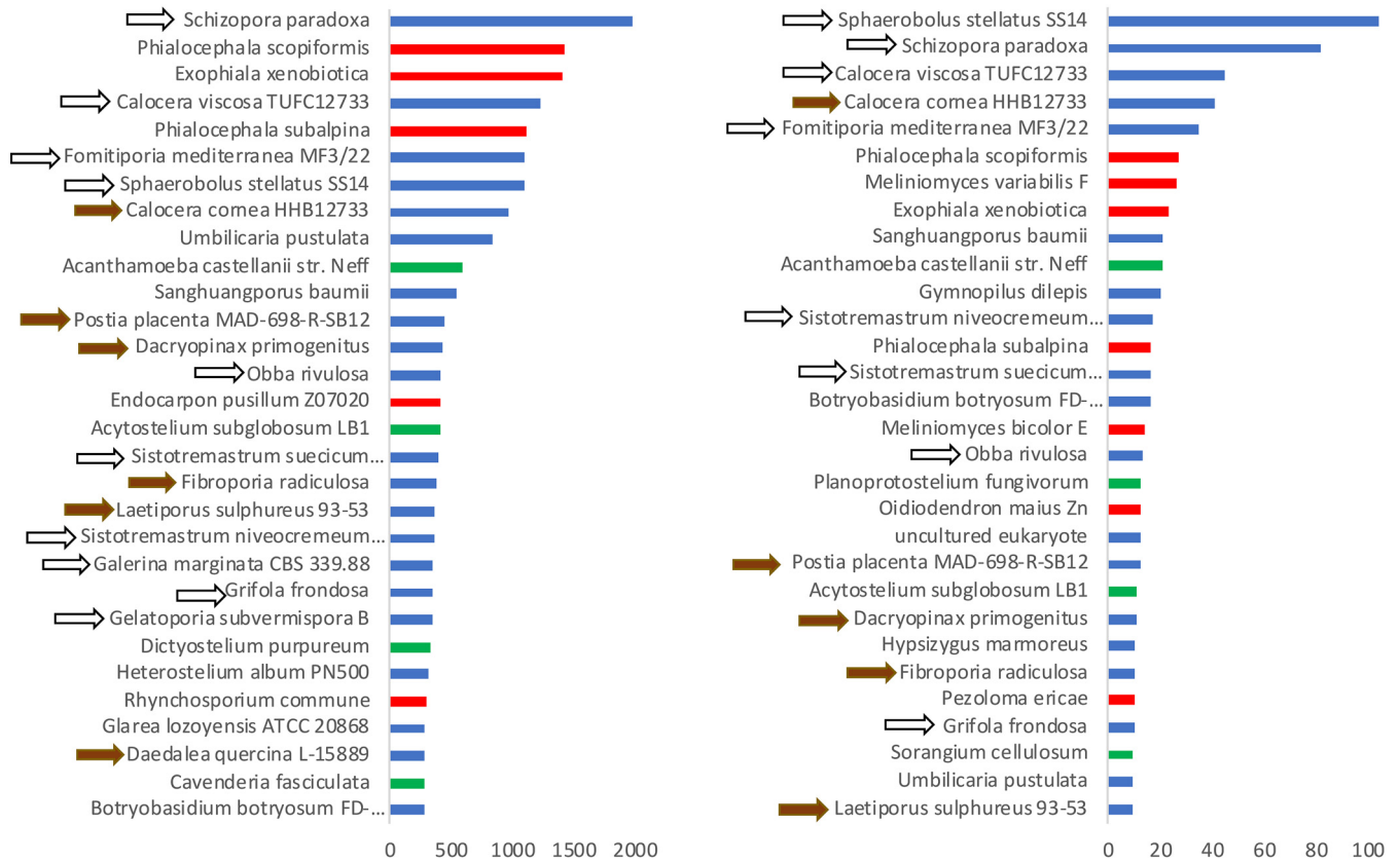
FIG 5 Distributions of top 30 BLASTp (NR database) hits among translations of all 52,011 contigs (left) and for 1,316 contigs (right) identified as CAZyme encoding. The 30 species account for 43% and 54% of the total top hits for all proteins and the CAZyme subset, respectively. White and brown arrows indicate decay type, where known. Fill colors correspond to Basidiomycota (blue), Ascomycota (red), and various other eukaryotes or bacteria (green).
