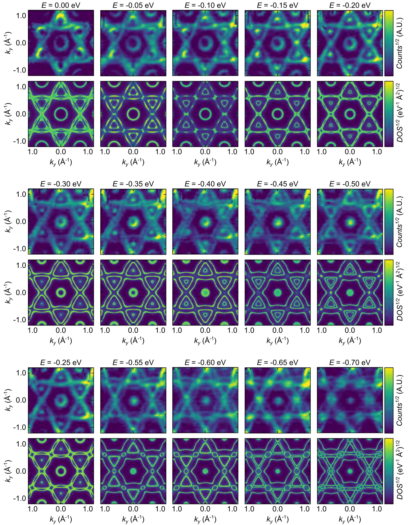
SFig 9. Additional angle-resolved photoemission spectroscopy (ARPES) data of \text{CsV}_3\text{Sb}_5 collected in increments of 0.05 eV from the Fermi energy to -0.7 eV. Excellent agreement is found between experimental data (top panels) and tight-binding models (bottom panels) over all energies.
