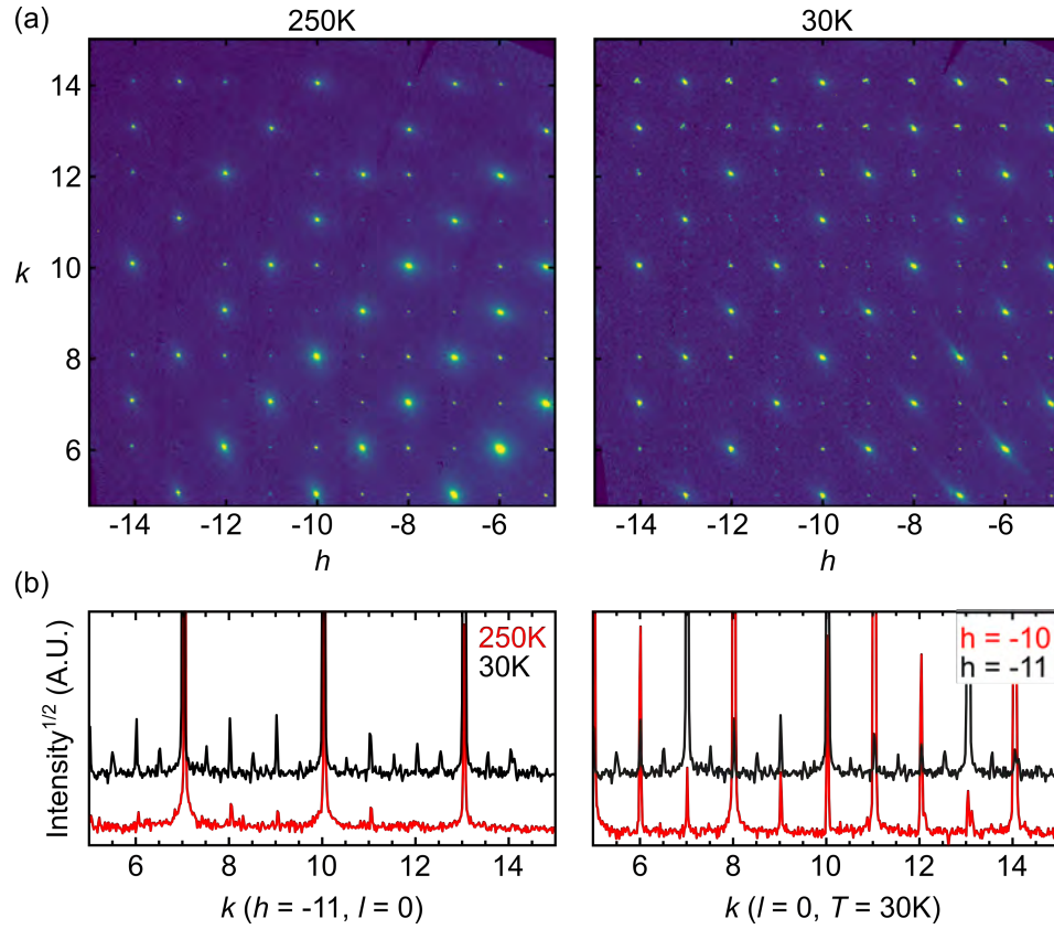
SFig 6. Synchrotron x-ray diffraction on single crystals of \text{CsV}_3\text{Sb}_5 reveal superlattice peaks upon cooling through the T^* = 94 K transition. (a) 2-D slices through Q -space showing the (h, k, 0) diffraction plane at T = 250 K and T = 30 K. Faint superlattice peaks appear at half integer positions below the 94K transition. Note that the data is plotted on a rectangular grid. (b) Line cuts through (h, k, 0) maps showing the appearance of superlattice peaks with decreasing temperature (left) and their dependence on the parity of h and k values (right). Diffraction data identifies superlattice peaks predominately appear at half-integer, odd, h/k values.
