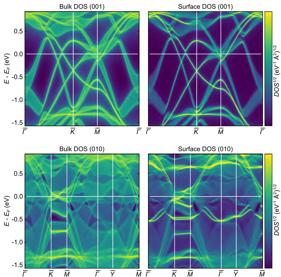
SFig 10. Tight-binding models were fit to DFT data, allowing a comparison of the bulk density of states and surface density of states on the (001) and (010) surfaces of CsV 3 Sb 5 . Comparing the bulk and surface DOS, a myriad of surface states can be seen throughout the electronic structure. The main body focuses on the time reversal invariant momentum (TRIM) point about 0.05 eV above the Fermi energy, although there are many other candidate states below the Fermi energy as well.
