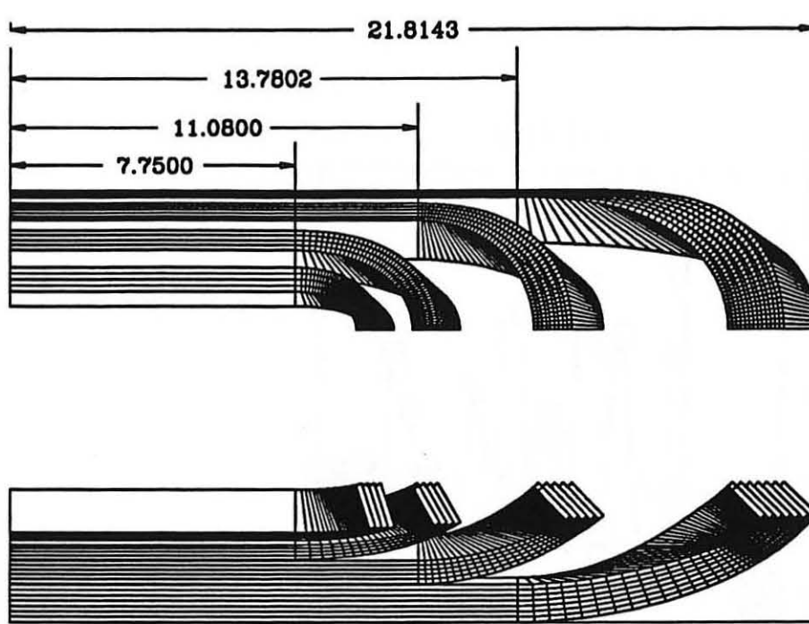
Figure 21 Conductor geometry in the end region of Dipole D19 — LAYER-1, TOP and SIDE view.
