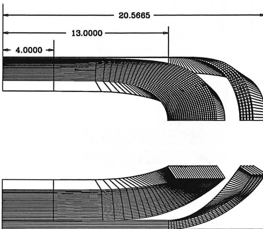
Figure 21 Conductor geometry in the end region of Dipole D19 — LAYER-1, TOP and SIDE view.
