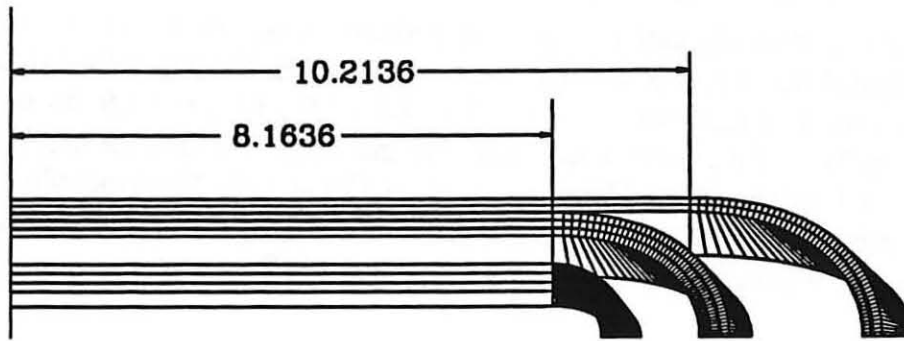
Figure 11 Conductor geometry in the end region of the SSC quad — LAYER-1 TOP.
