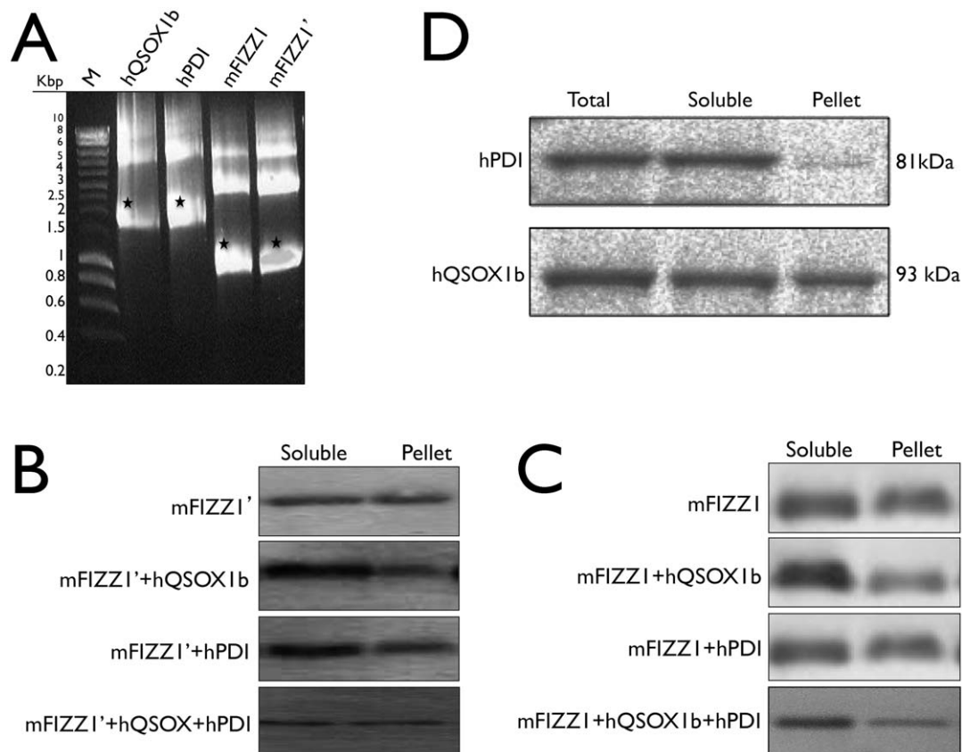
Figure 3. Co-expression with hQSOX1b increased the soluble expression of mFIZZ1. (A) Ethidium bromide stained agarose gel with the mRNA of hQSOX1b, hPDI, mFIZZ1 and mFIZZ1' after transcription is shown. (B) An immunoblot developed with anti-His antibody shows the expression of mFIZZ1' without thiol-disulfide oxidoreductase, with hQSOX1b, with hPDI and with hQSOX1b + hPDI. (C) An immunoblot developed with anti-His antibody shows the expression of mFIZZ1 without thiol-disulfide oxidoreductase, with hQSOX1b, with hPDI and with hQSOX1b + hPDI. (D) An immunoblot developed with anti-GST antibody shows the expression of both hQSOX1b+GST (93 kDa) and hPDI+GST (81 kDa) after the co-expression reaction with mFIZZ1.
