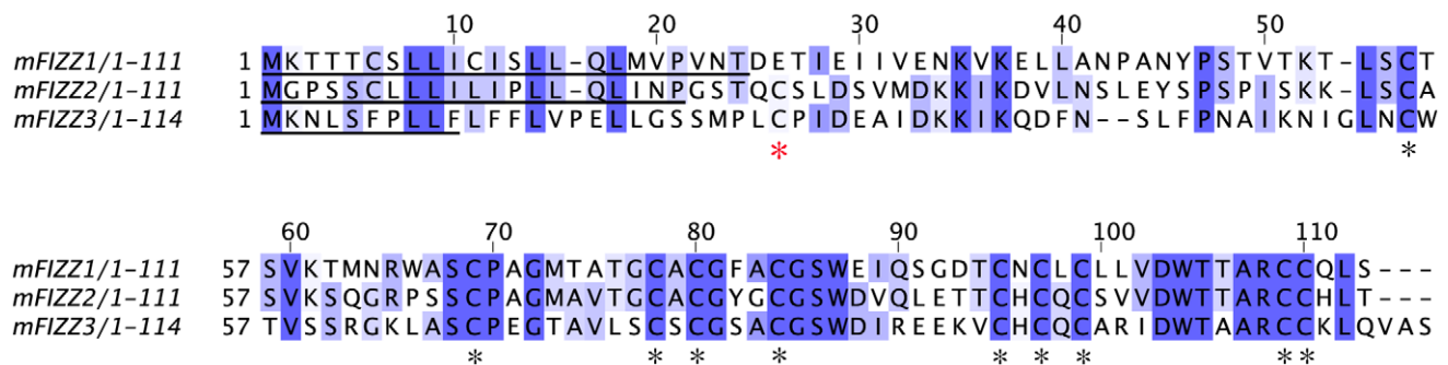
Figure 1. The cysteines in the resistin family are highly conserved. A ClustalW alignment [50] of the mFIZZ protein amino acid sequences is shown. Gene Bank accession numbers are for mFIZZ1, AF205951; mFIZZ2, Q99P86 and mFIZZ3 Q99P87. The conserved residues have been coloured in blue grade (conservation level 30%). The conserved cysteines are marked with black asterisks, and the signal peptides are underlined. The position of the extra N-terminal cysteine in mFIZZ2 and mFIZZ3 is indicated with a red asterisk. The extra N-terminal cysteine is thought to be involved in an inter-molecular disulfide bond in mFIZZ2 [27]. doi:10.1371/journal.pone.0055621.g001
