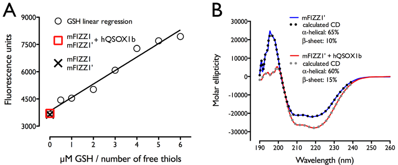
Figure 5. mFIZZ1' has a high helical content and all the intramolecular disulfide bonds are formed. (A) The results of a Thiostar assay using glutathione as a standard are shown. mFIZZ1' and mFIZZ1 prepared with and without hQSOX1b show no free thiols. (B) The CD-spectrum of mFIZZ1' produced with and without hQSOX1b showed a double minimum at 208 and 222 nm characteristic for \alpha -helical proteins. doi:10.1371/journal.pone.0055621.g005
