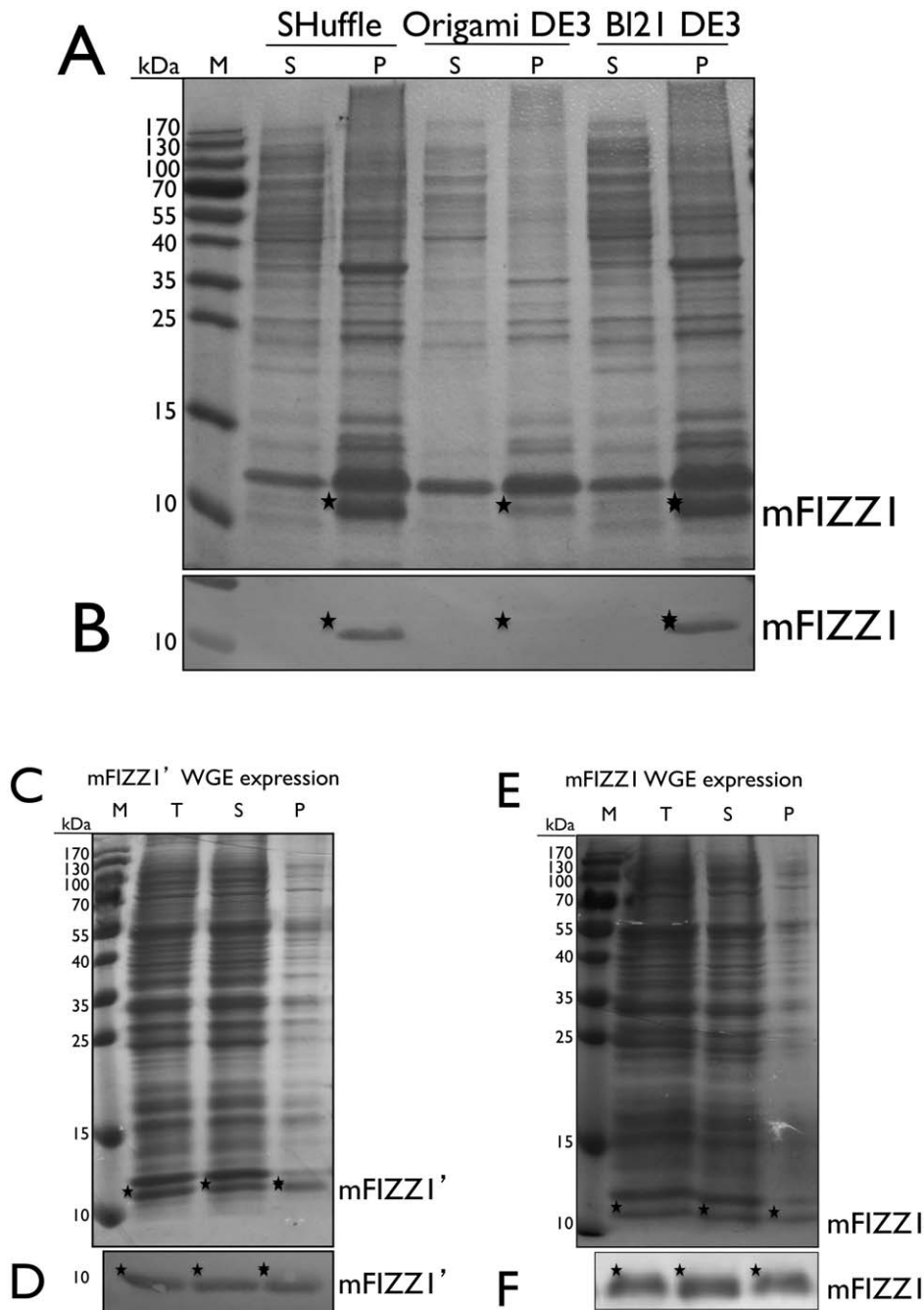
Figure 2. mFIZZ1 soluble expressed using wheat germ extract. (A) The expression of mFIZZ1 in SHuffle™ T7, Origami DE3 and BL21 DE3 analysed on non-reducing 15% SDS-PAGE stained with Coomassie Brilliant Blue. (B) Strip of the immunoblot from the SDS-PAGE in (A) developed with anti-His antibody is shown. (C) The expression of mFIZZ1' with wheat germ extract analysed on non-reducing 15% SDS-PAGE stained with Coomassie Brilliant Blue. (D) Strip of the respective immunoblot of (C) developed with anti-His antibody is shown. (E) The expression of mFIZZ1 with wheat germ extract analysed on non-reducing 15% SDS-PAGE stained with Coomassie Brilliant Blue. (F) Strip of the respective immunoblot of (E) developed with anti-His antibody is shown. As marker (M) the PageRuler™ pre-stained Protein Ladder (Fermentas) is used. P=pellet, S=soluble fraction and T=total. The corresponding bands are indicated with an asterisk. doi:10.1371/journal.pone.0055621.g002
