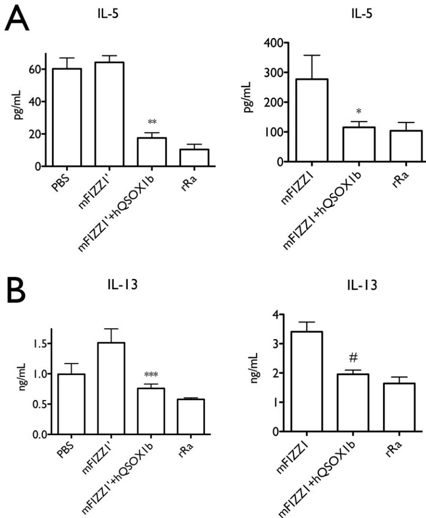
Figure 6. mFIZZ1' and mFIZZ1 decreased the IL-13 and IL-5 secretion of splenocytes. Splenocytes were cultured at 200,000 cells/well and activated under Th2 permissive conditions for 4 days. Recombinant mFIZZ1' and mFIZZ1 expressed with or without hQSOX1b were used at 200 ng/ml. rRa is the bacterial recombinant FIZZ1 (200 ng/ml) from (Peprotech) and PBS is the control. (A) Recombinant mFIZZ1' and mFIZZ1 co-expressed with hQSOX1b significantly decreased the IL-5 secretion compared to the proteins expressed alone. (B) Recombinant mFIZZ1' and mFIZZ1 co-expressed with hQSOX1b decreased the IL-13 secretion compared to the proteins expressed alone. *** P < 0.001 ; ** P < 0.01 ; * P < 0.05 ; # P = 0.07 . Results are representative of three independent experiments for mFIZZ1' and two independent experiments for mFIZZ1, and statistical analysis was performed by two-way ANOVA.
