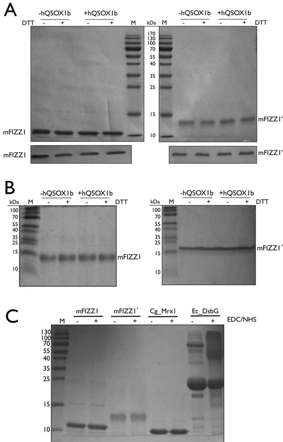
Figure 4. mFIZZ1 and mFIZZ1' are highly pure and monomeric. (A) CBB-stained 15% SDS-PAGE of the purified mFIZZ1' and mFIZZ1 co-expressed with and without hQSOX1b under reducing and non-reducing conditions followed by immunoblot developed with anti-His antibody. The samples are highly pure and proteins migrate at the same position under reducing and non-reducing conditions, indicating that no intermolecular disulfide bonds are formed. (B) Basic native PAGE of the purified mFIZZ1 and mFIZZ1' co-expressed with and without hQSOX1b under reducing and non-reducing conditions. The protein bands for mFIZZ1 (pI 4.81) and mFIZZ1' (pI 5.18) migrate on a slightly different position due to their pI. No major multimeric bands are observed. (C) A CBB-stained 15% non-reducing SDS-PAGE of mFIZZ1 and mFIZZ1' co-expressed with hQSOX1b after cross-linking with a mixture EDC/NHS for 3 h at room temperature is shown. As negative and positive controls, monomeric Corynebacterium glutamicum mycoredoxin-1 (Cg_Mrx1) and dimeric Escherichia coli DsbG (Ec_DsbG) were used. Monomeric Cg_Mrx1 migrates after crosslinking as monomer. For dimeric Ec_DsbG (present as a mixture between monomer and dimer on SDS-PAGE), bands shift from the monomeric and the dimeric migration position to a higher molecular weight positions. For both mFIZZ1 and mFIZZ1' no shift to a higher molecular weight is observed. As marker (M) in panels A, B and C, the PageRuler™ pre-stained Protein Ladder (Fermentas) is used, which contains SDS. doi:10.1371/journal.pone.0055621.g004
