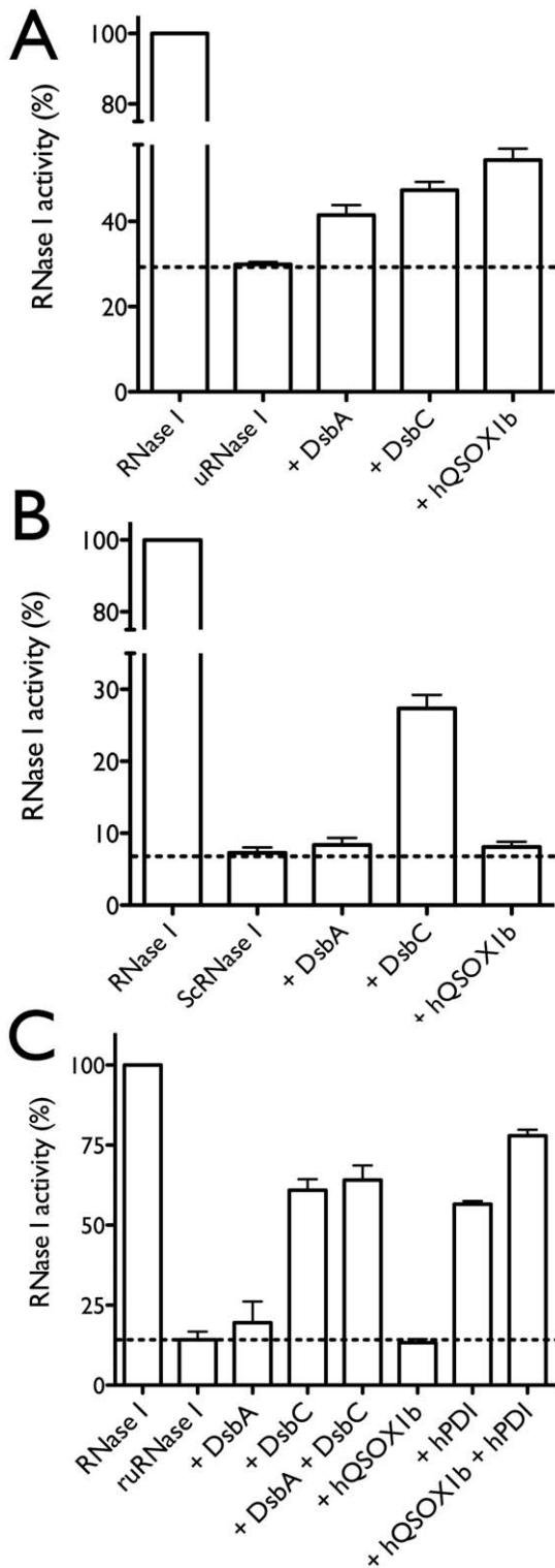
Figure 7. hQSOX1b has chaperone activity and cooperates with PDI to fold reduced unfolded RNase I. The mean values and the standard deviation of the RNase I activity of three independent experiments are shown. (A) Chaperone assay with unfolded RNase I (uRNase I). hQSOX1b helps to fold unfolded RNase I (B) Isomerase assay with scrambled RNase I (scRNase I). hQSOX1b did not show isomerase activity, while the isomerase DsbC partially rescues the RNase I activity. (C) Oxidase assay with reduced unfolded RNase I (ruRNase I). Combining hQSOX1b with hPDI, and DsbA with DsbC results in the highest oxidative folding efficiency. hQSOX1b on its own does not
