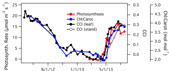
Fig. 2. Seasonal patterns of leaf photosynthesis, leaf chlorophyll/carotenoid pigment ratios, and the CCI at the leaf (solid black line) and stand (dotted line and open circles) scales. All data were from P. contorta (lodgepole pine) seedlings grown in Alberta, Canada.
