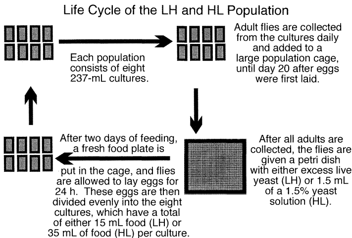
FIG. 1. The life cycle of the experimental LH and HL populations. The population represented by this figure is just one of the 20 experimental populations.
