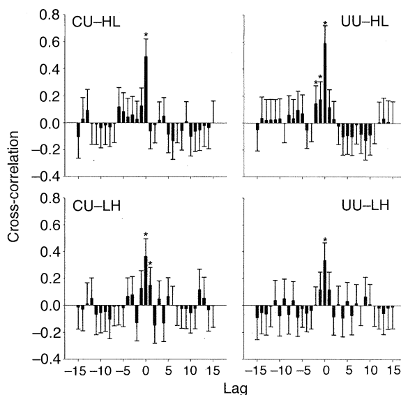
FIG. 5. The cross-correlation between adult numbers and the inverse of per capita mass with 95% confidence intervals. A lag of m positive units means that a correlation of adult numbers at time t is computed with (i.e., lagged with) the inverse mass at time t + m . Confidence intervals were estimated as in Fig. 4, from the replicate populations.
