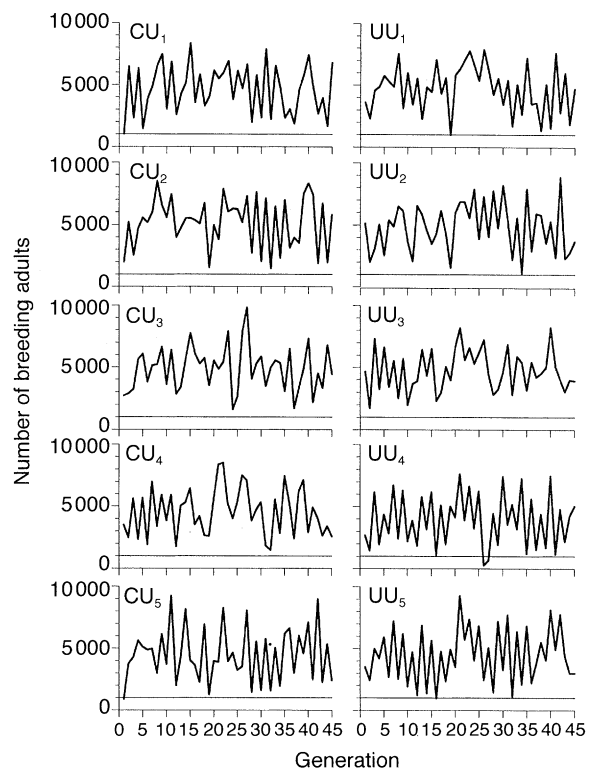
FIG. 3. The total adult population size in each of 10 LH experimental populations, over 45 generations. Each population was censused immediately after reproduction. A horizontal line in each figure shows how infrequently population size dipped below 1000 adults.
