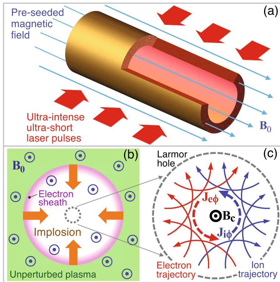
Figure 1. (a) Perspective view of a microtube irradiated by ultraintense laser pulses (laser configuration is just schematic). Uniform external magnetic field B_0 is pre-seeded prior to main laser illumination. (b) Top view of the inner plasma dynamics. Laser-produced hot electrons drive isothermal expansion of the inner-wall plasma into vacuum. (c) Ultrahigh magnetic field B_c is generated at the center due to the collectively formed currents by ions and electrons, which are deflected in opposite directions by B_0 .
