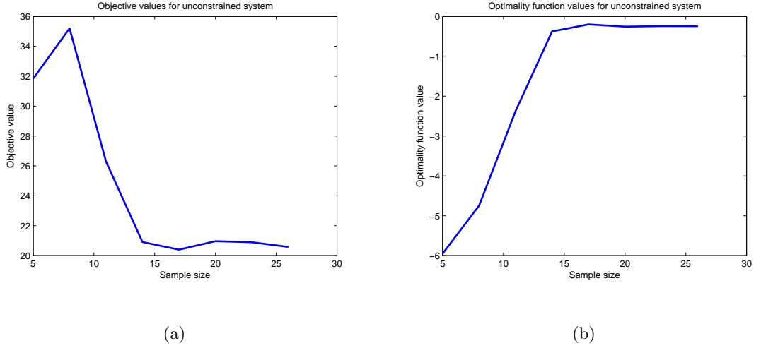
Figure 4.3: a) The value of the objective functional (4.22) for Problem S_O computed using sample averages, as a function of the sample size M . b) The value of the optimality function (4.26) as a function of the sample size M .
