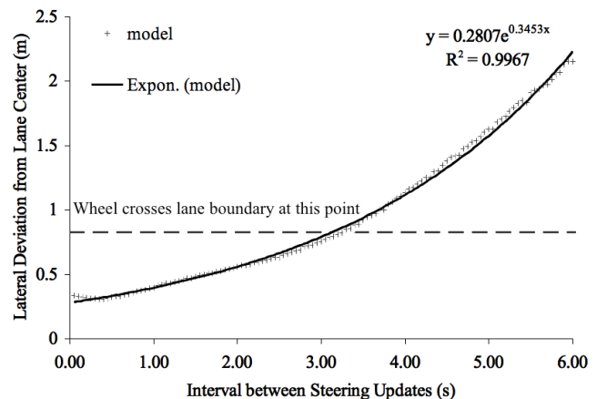
Figure 1 Data plot showing relationship between steering update interval and average lateral deviation.
