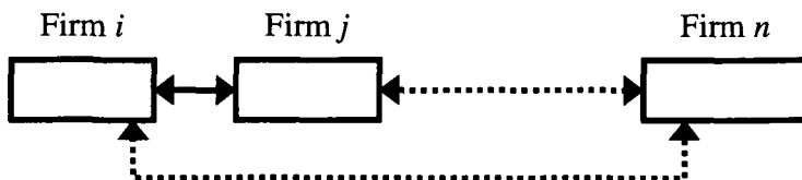
FIGURE 2: CROSS-HOLDINGS
