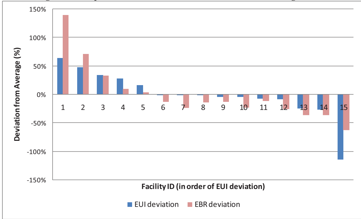
Figure 3. Comparison of Filter- And Model-Based Benchmarking Results
