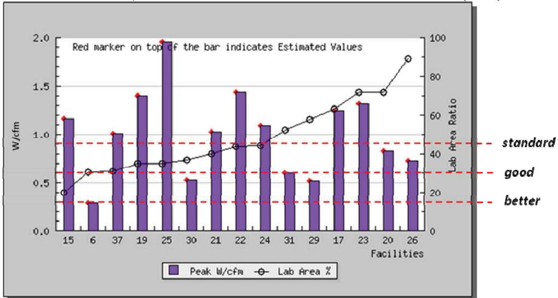
Figure 5. Ventilation W/cfm Data from the Labs21 Benchmarking Database. Benchmarks for Standard, Good and Better Practice Are Based on Labs21 (2005)
