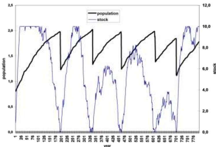
Figure 2. Example of calculation using this model for r^0 = 1.02 , p^0 = 2 , a_0 = 2 , a_1 = 1.2 , p_1 = 1.05 .
