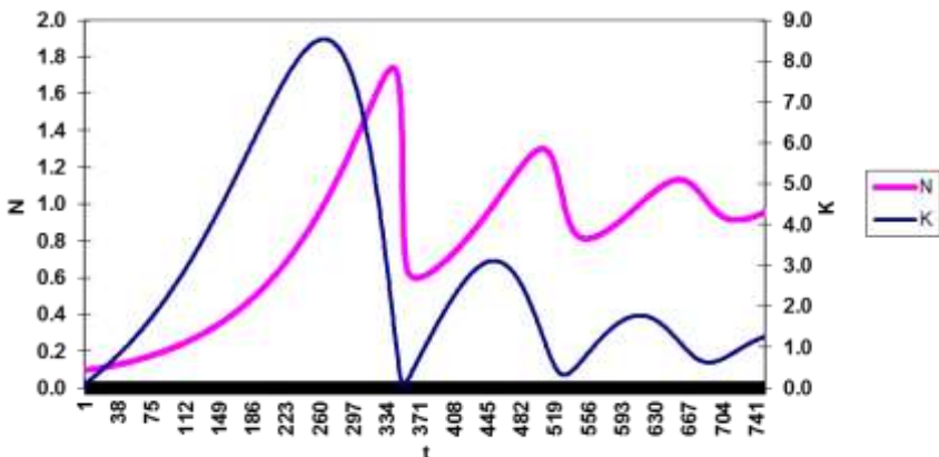
Figure 1. Example of calculations using the model ( r=0.01 ; p=1.2 )
