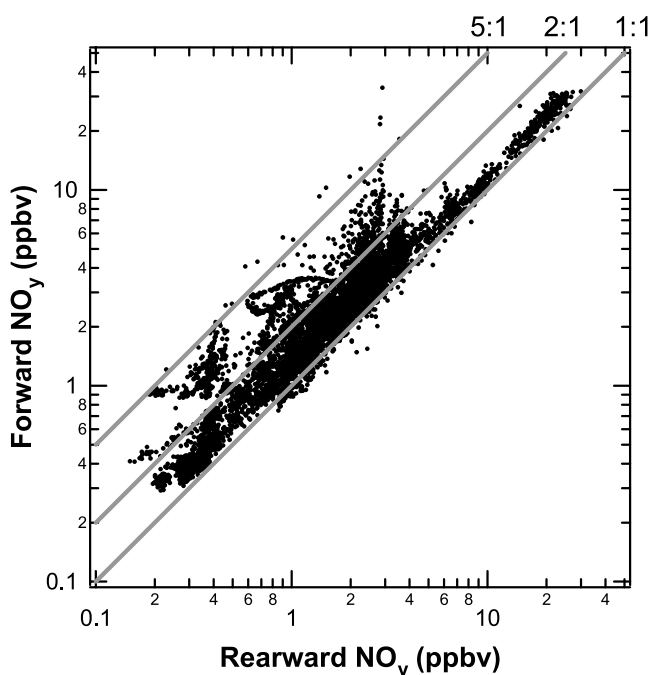
Figure 2. Correlation of NO y mixing ratios measured using the forward facing inlet (forward NO y ) and those using the rearward facing inlet (rearward NO y ). The data points are 1-s averages and represent the entire data set used in this analysis. Shaded lines indicate 1:1, 2:1, and 5:1 correspondence lines.
