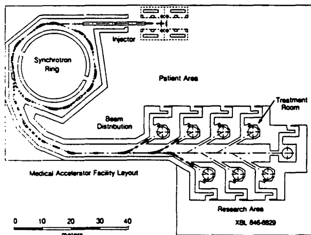
Fig. 1 Medical Accelerator Layout
