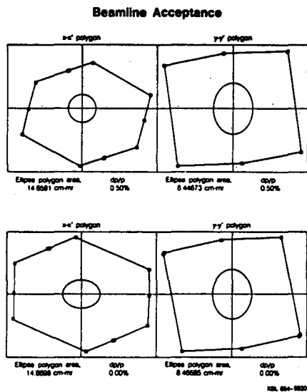
Fig. 5 Beamline Acceptance
