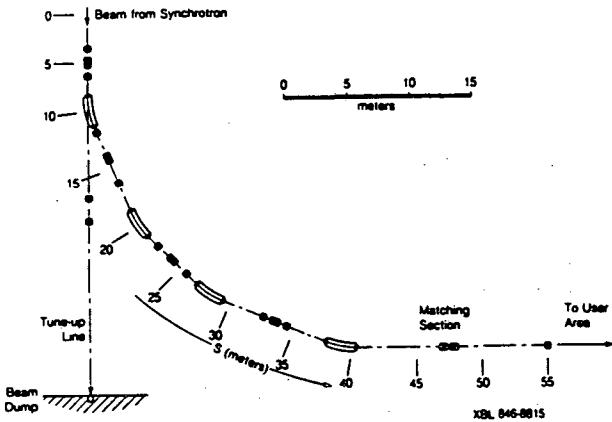
Fig. 2 90° Bend Section Layout
