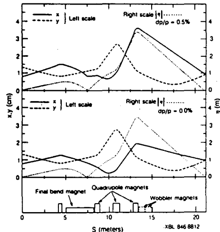
Fig. 4 Beam User Area Optics and Layout
