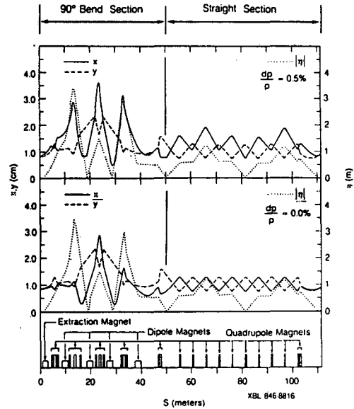
Fig. 3 Beamline Optics
