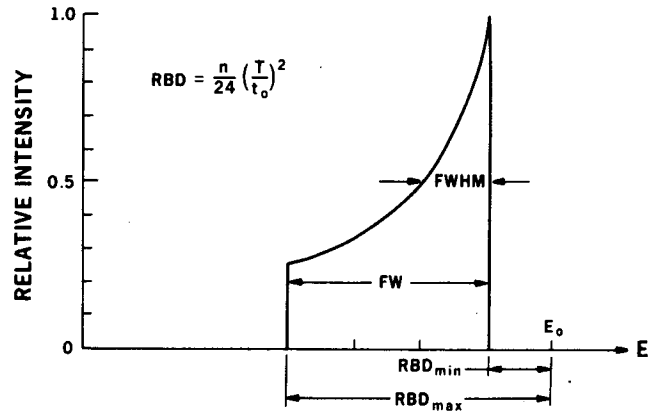
Fig. 4. Asymmetrical Spectral Broadening Due to Ballistic Deficits.
