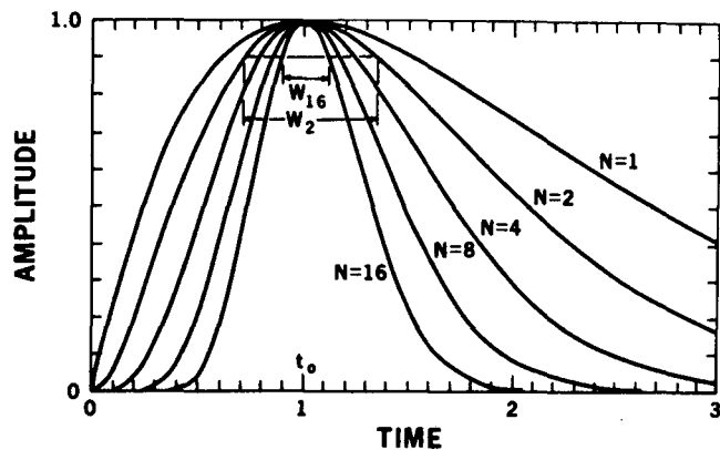
Fig. 3 Semi-Gaussian Shaping Functions of Order N Normalized to the Peaking Time t_0 . The W 's are the Full Width at 90% Maximum Values.
