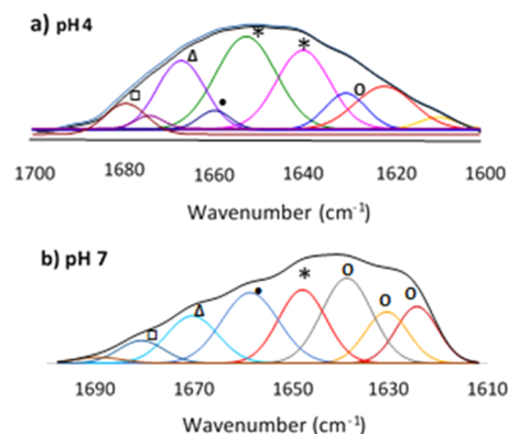
Figure 6. ATR-FTIR spectra of 1 mg/mL Mfp3F in deuterated buffer at (a) pH 4 and (b) pH 7: (○) \beta -sheet, (*) random coil, (●) \alpha -helix, (Δ) 3_{10} helix, and (□) turns. Secondary derivatives are shown in the Supporting Information (S 9 ).
