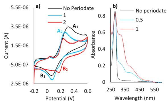
Figure 1. (a) CV of the CPE electrode in 5 \times 10^{-5} M D in 0.1 M PBS (pH 7), with a scan rate of 0.05 \text{ V s}^{-1} . (b) UV-vis spectra for oxidation of 8 \times 10^{-4} M D in 0.1 M PBS (pH 7). The blue curve in panel a) denotes a 1:1 periodate:Dopa ratio, whereas the red curve denotes a 2:1 ratio. In panel b), the blue and red curves denote 0.5:1 and 1:1 periodate: Dopa ratios, respectively.
