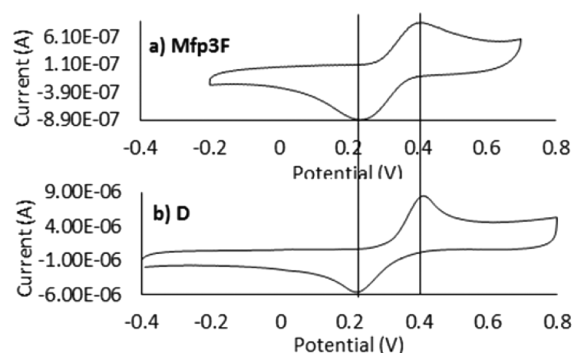
Figure 4. CVs of (a) Mfp3F and (b) D in 0.1 M acetate buffer (pH 4), with a scan rate of 0.05 \text{ V s}^{-1} .
