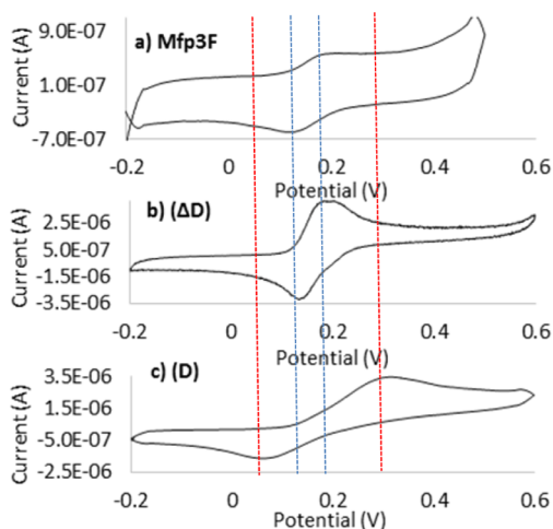
Figure 5. CVs of (a) Mfp3F, (b) purified \Delta D , and (c) D in 0.1 M PBS (pH 7), with a scan rate of 0.05 \text{ V s}^{-1} .
