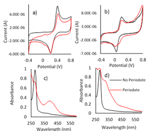
Figure 3. CV of the CPE electrode in D ( 5 \times 10^{-5} \text{ M} ) (a) in acetate buffer (pH 4) and (b) in 0.1 M PBS (pH 8). UV-vis spectra for oxidation of D ( 8 \times 10^{-4} \text{ M} ) (c) in acetate buffer (pH 4) and (d) in 0.1 M PBS (pH 8), with a scan rate of 0.5 \text{ V s}^{-1} .
