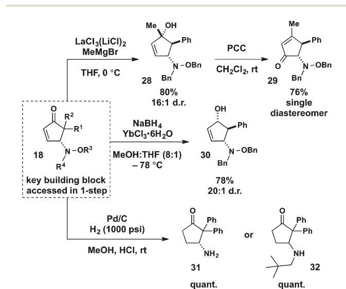
Scheme 2 Selected functionalization of the cyclopentenone scaffold. The relative stereochemistry of 28 was assigned by analogy to 30 .
