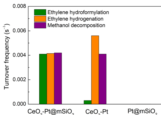
Figure 3. Ethylene hydroformylation with methanol carried out at 150 °C over \text{CeO}_2\text{-Pt@mSiO}_2 and single interface catalysts \text{CeO}_2\text{-Pt} and \text{Pt@mSiO}_2 . Methanol, ethylene, and helium partial pressures were 35, 7.5, and 727.5 Torr, respectively.
