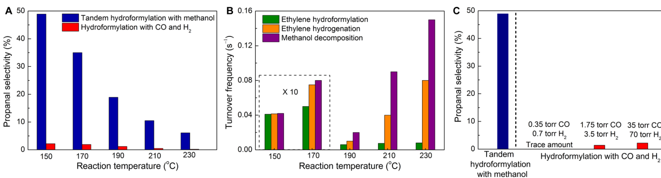
Figure 4. Catalytic performance of \text{CeO}_2\text{-Pt@mSiO}_2 for the hydroformylation of ethylene with methanol at an ethylene pressure of 7.5 Torr. (A) Comparison of tandem hydroformylation of ethylene with methanol and single-step hydroformylation with CO and \text{H}_2 . (B) The influence of temperature on tandem hydroformylation of ethylene. (C) Catalytic performance of single-step hydroformylation under a deficiency of CO and \text{H}_2 at 150 °C.
