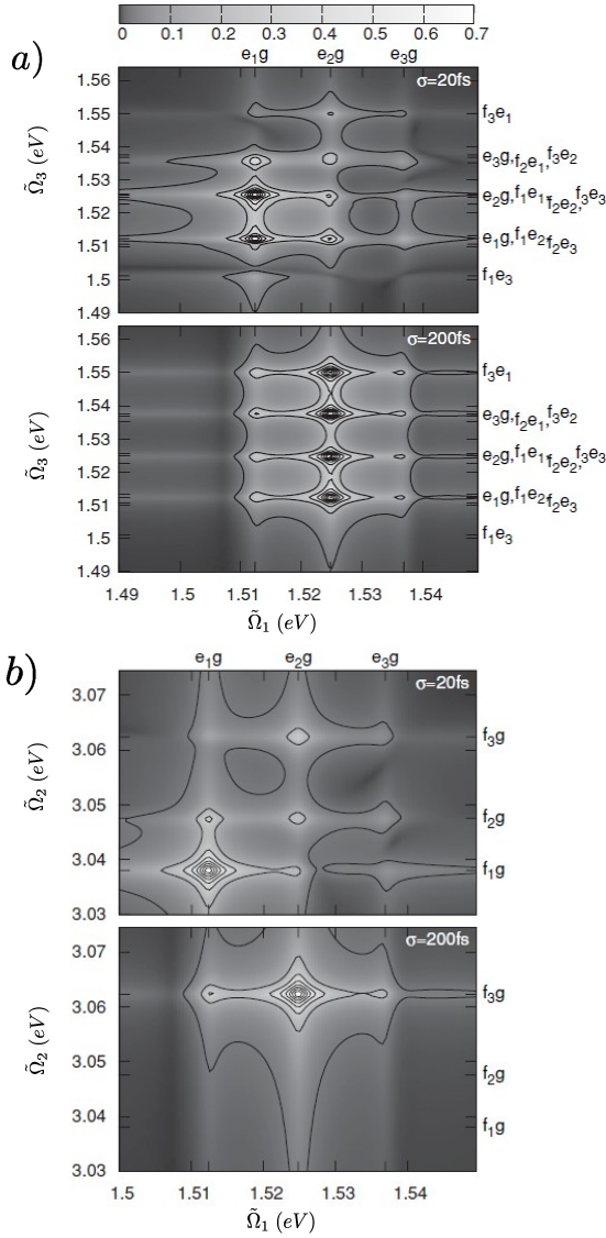
FIG. 20 (Color online) a) 2D signal S_{DQC}^{(LAP)}(\tilde{\Omega}_1, \tilde{\Omega}_3) Eq. (162) (absolute value), showing correlation plots with different pump bandwidths \sigma as indicated. The bottom panel is multiplied by x6. b) Same as a) but for 2D signal S_{DQC}^{(LAP)}(\tilde{\Omega}_1, \tilde{\Omega}_2) Eq. (163). Parameters for simulations are given in Ref. (Richter and Mukamel, 2010).
