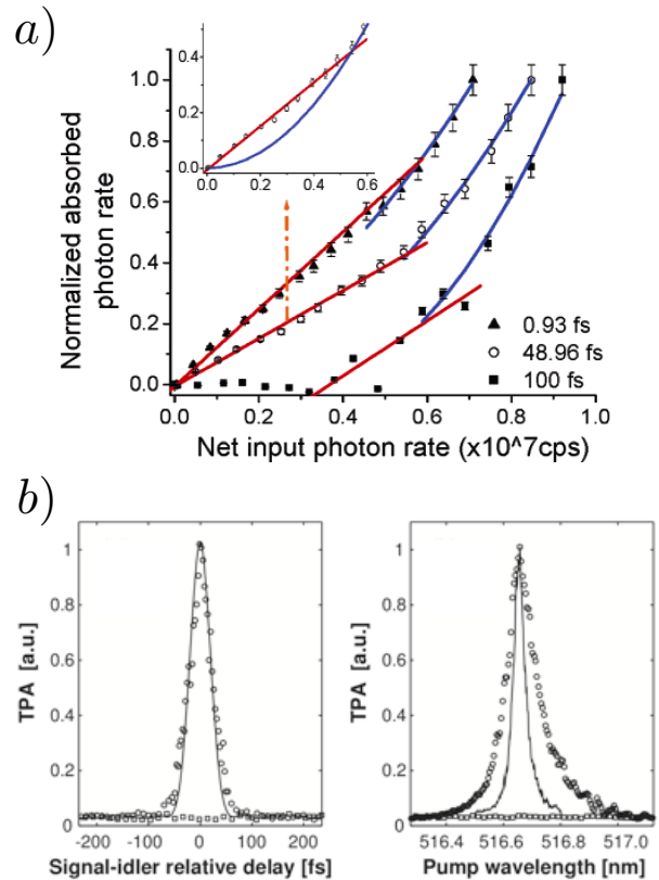
FIG. 1 a) Linear entangled TPA rate and quadratic nonlinear random TPA rate in a porphyrin dendrimer at different entanglement times. The inset shows the dominant effect of the entangled TPA at low input flux of correlated photons. b) Two-photon absorption 5S_{1/2} \rightarrow 4D_{5/2,3/2} in atomic Rubidium (Dayan et al. , 2004) vs. the time delay between the two photons (left panel), and vs. the pump frequency (right panel).
