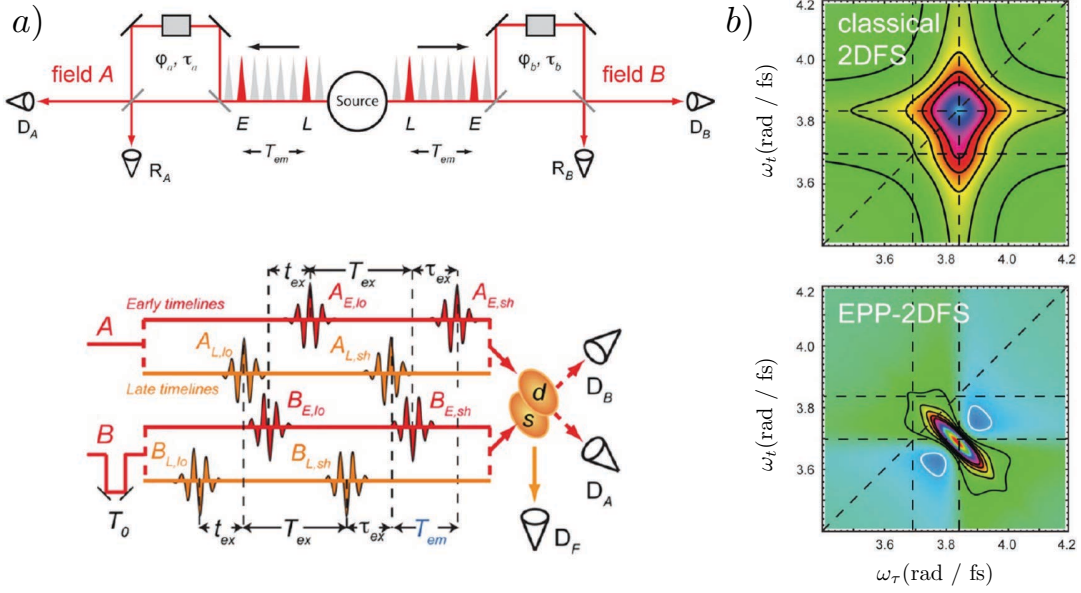
FIG. 15 a) Experimental setup for the LOP protocol: By sending each beam through a Franson interferometer, the photon excitation may occur either via a delayed or an “early” photon. b) Top panel: two-dimensional fluorescence spectrum induced by classical light. Bottom panel: the same spectrum induced by entangled photons. [taken from (Raymer et al. , 2013)]
