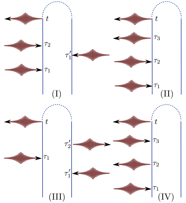
FIG. 19 Diagrams representing the third-order contributions to Eq. (131).
