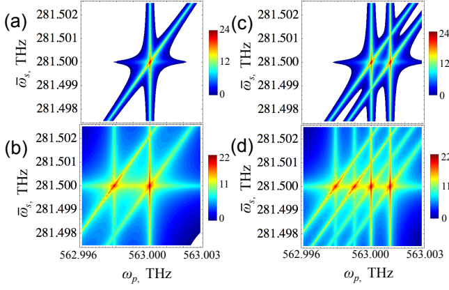
FIG. 34 (Color online) Left column: two dimensional PCC rate (log scale in arb. units) calculated using quantum theory Eq. (175) assuming a single monochromatic pump with frequency \omega_p . Idler detector resonant with intermediate level \bar{\omega}_i = \omega_{eg} = 282\text{THz} - (a), while \omega_{eg} - \bar{\omega}_i = 2\text{GHz} for (b). Right column: same as left but for a pump made out of two monochromatic beams with frequencies \omega_p - \omega'_p = 2 \cdot 10^{-6}\omega_p .
