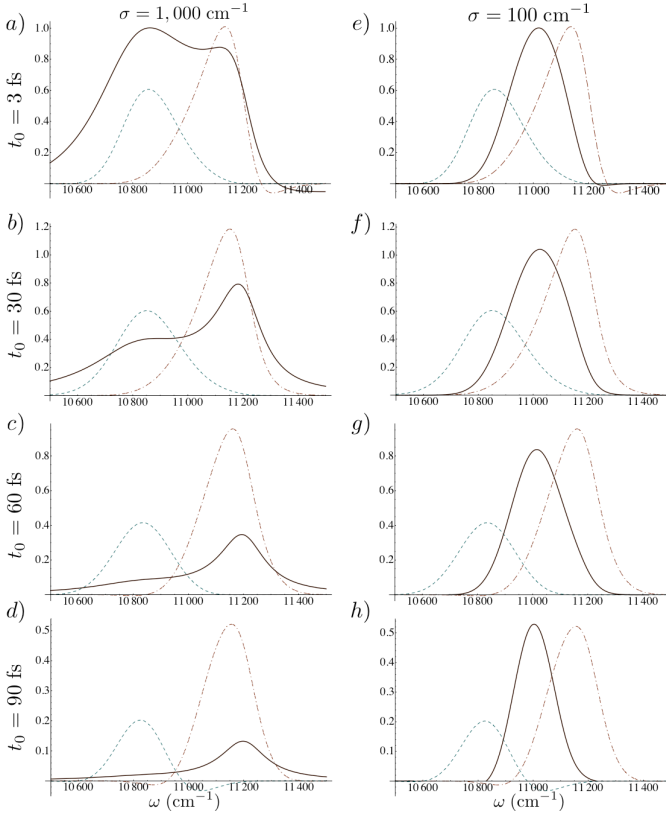
FIG. 24 (Color online) a) TPC signals with \sigma_p = 2,000 \text{ cm}^{-1} and T = 90 \text{ fs} , \omega_r = 10,400 \text{ cm}^{-1} (blue, dashed) and 11,400 \text{ cm}^{-1} (red, dot-dashed) as well as the classical pump-probe signal (black, solid) with \sigma = 1,000 \text{ cm}^{-1} are plotted vs. the dispersed frequency \omega with a time delay set to t_0 = 3 \text{ fs} . b) Same for t_0 = 30 \text{ fs} , c) 60 \text{ fs} , d) 90 \text{ fs} . e)-h) Same as a)-d), but with classical bandwidth \sigma = 100 \text{ cm}^{-1} . The classical signal is normalized, such that its maximum value at t_0 = 0 is equal to one. Similarly, the TPC signal are normalized to the maximum value of the signal with \omega_r = 11,400 \text{ cm}^{-1} at t_0 = 0 . [taken from (Schlawin et al. , 2015)]
