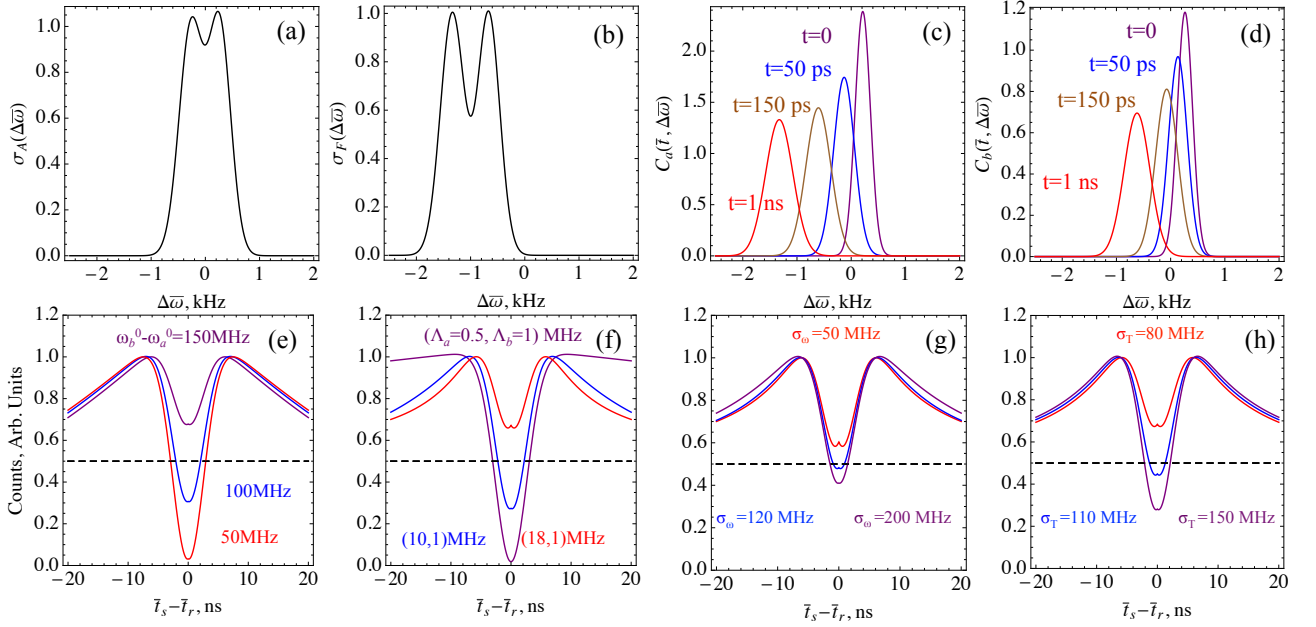
FIG. 35 (Color online) Top row: Absorption (276) - (a) and fluorescence (277) - (b) line shapes vs displaced frequency \Delta\bar{\omega} = \omega - \frac{1}{2}(\omega_a + \omega_b) . Frequency dispersed time-resolved fluorescence (284) displayed as a snapshot spectra for molecule a - (c) and b - (d). Bottom row: PCC for different transition energies of molecules excited at \omega_p = \omega_b^0 + \lambda_b - (e); PCC for different values of the SD time scale \Lambda_a and \Lambda_b and fixed linewidth \Gamma_a, \Gamma_b according to Eq. (275) - (f); PCC for different frequency gate bandwidths - (g) at fixed time gate bandwidth \sigma_T = 100 MHz and for different time gate bandwidths - (h) at fixed frequency gate bandwidth \sigma_\omega = 100 MHz. Molecules have distinct SD timescales \Lambda_a = 15 MHz, \Lambda_b = 1 MHz and \omega_b^0 - \omega_a^0 = 1 MHz.
