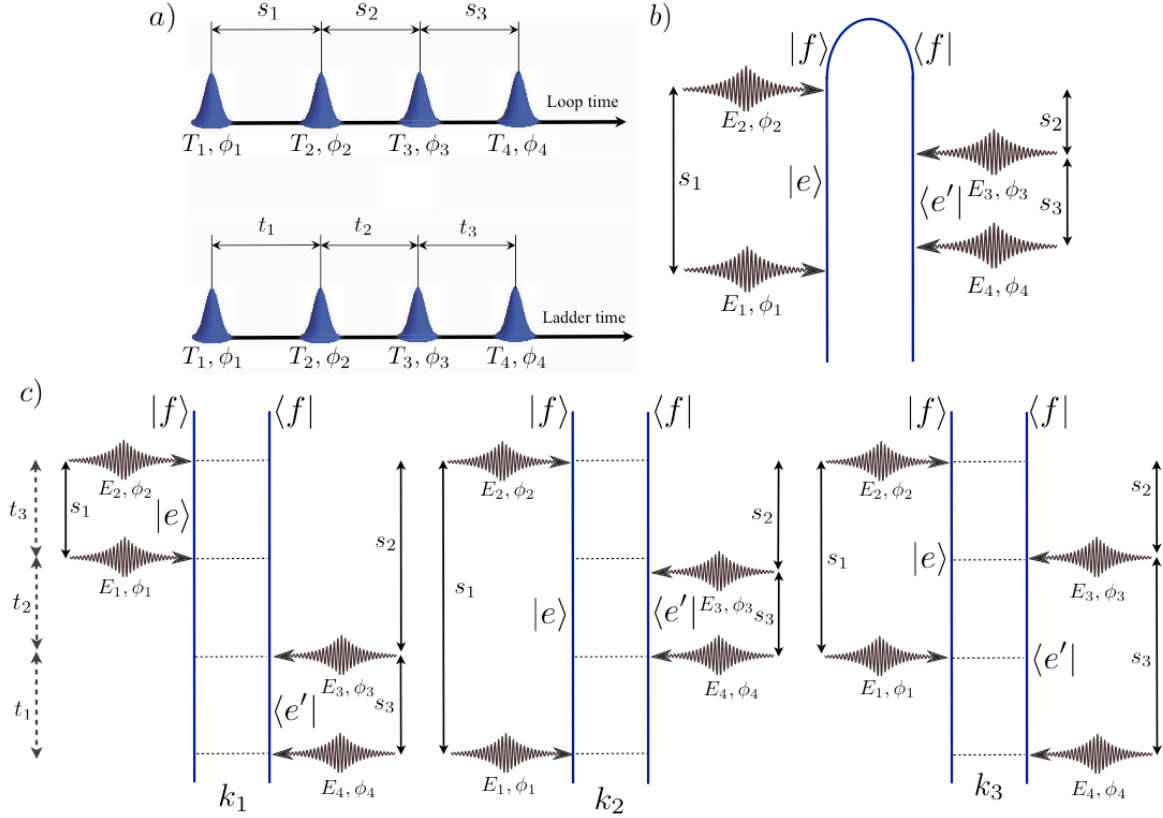
FIG. 16 (Color online) a) Pulse sequence for LOP (top panel) and LAP (bottom panel) scanning protocols. b) Loop diagram for the TPA process with indicated loop delays for the non specified phase cycling that depends on chronological time ordering between pulses 1 to 4 c). Ladder diagrams for the TPA signal with selected phase cycling component corresponding to double quantum coherence term k_I : -\phi_d - \phi_c + \phi_b + \phi_a , rephasing k_{II} : -\phi_4 + \phi_2 + \phi_1 - \phi_3 , and nonrephasing k_{III} : -\phi_4 + \phi_2 - \phi_3 + \phi_1 . Both loop s_j and ladder t_j delays, j = 1, 2, 3 are indicated. The transformation between two is different for each diagram. Time translation invariance implies \omega_1 + \omega_2 - \omega_3 - \omega_4 = 0 .
