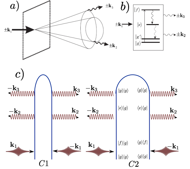
FIG. 31 Three wave process involving two quantum and one classical mode: (A) phase-matching condition; (B) molecular level scheme; (C) loop diagrams for the incoherent TPEF (C1) and coherent Type I PDC (C2)
