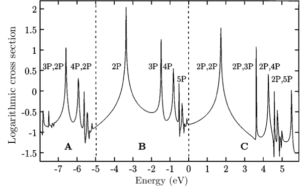
FIG. 12 Entangled virtual-state spectroscopy: TPIF signal vs. the Fourier transform of an additional time delay between the two photons (see text) in hydrogen [taken from (Saleh et al. , 1998)].
