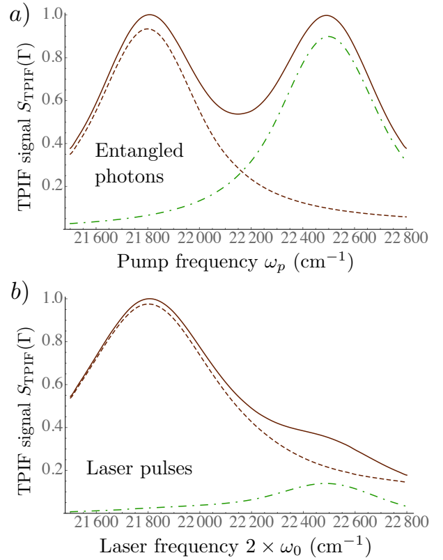
FIG. 13 a) TPIF action spectrum S_{\text{TPIF}}(\Gamma) , Eq. (114), induced by entangled photon pairs with the same parameters as in Fig. 10. The fluorescence created by the state f_1 is shown separately as a dashed plot, and the signal from f_2 as a dot-dashed line. b) TPIF action spectrum induced by laser pulses with bandwidth \sigma_0 = 100 \text{ cm}^{-1} .
