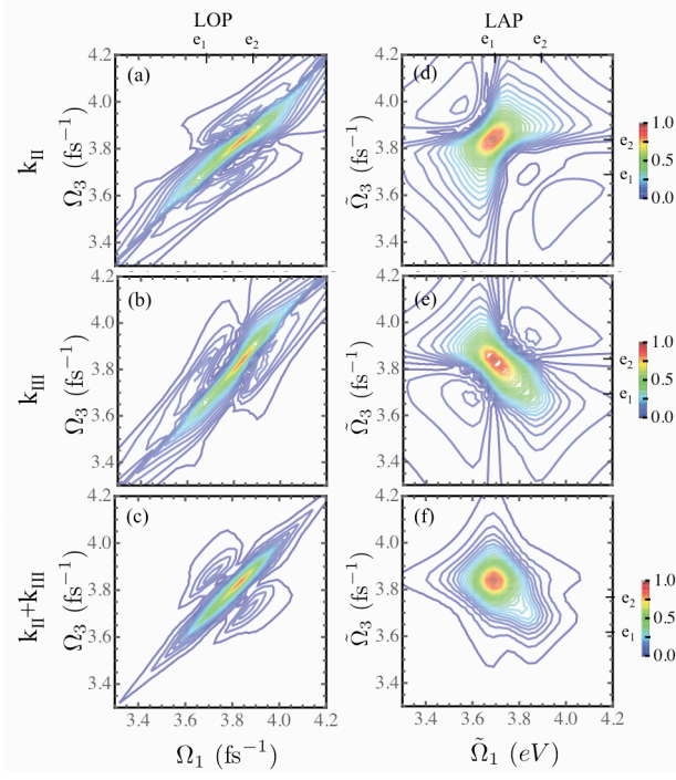
FIG. 17 (Color online) Left column: S_{LOP}(\Omega_1, \tau_2 = 0, \Omega_3) for the molecular dimer model of Ref. (Raymer et al. , 2013) calculated using classical light for rephasing \mathbf{k}_{II} Eq. (123) - (a), nonrephasing \mathbf{k}_{III} Eq. (124) - (b) and the sum of two \mathbf{k}_{II} + \mathbf{k}_{III} - (c). Right column: same for S_{LAP}(\tilde{\Omega}_1, t_2 = 0, \tilde{\Omega}_3) Eq. (119) - (120). Note that the the sum of rephasing and nonrephasing components for LAP signal we flipped the rephasing component to obtain absorptive peaks as is typically done in standard treatment of photon echo signals. The difference between the two columns stems from the display protocol and is unrelated to entanglement.
