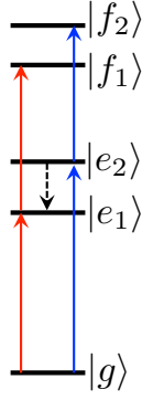
FIG. 8 Level scheme of the multilevel model employed in this review: Two singly excited states e_1 and e_2 with energies 11,000 \text{ cm}^{-1} and 11,500 \text{ cm}^{-1} are coupled to doubly excited states f_1 and f_2 , as indicated. Furthermore, e_2 decays to e_1 within 1/k \simeq 30 \text{ fs} .
