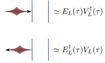
FIG. 37 Diagram construction in a QED formulation: The vertical blue lines indicate the evolution of the matter density matrix. An arrow pointing towards (away from) it corresponds to a matter excitation V^\dagger(\tau) (de-excitation V(\tau) ), which is accompanied by a photon annihilation E(\tau) [creation E^\dagger(\tau) ]. In the Liouville space formulation, interactions on the left side represent left-superoperators (1), and interaction on the right right-superoperators (2).
