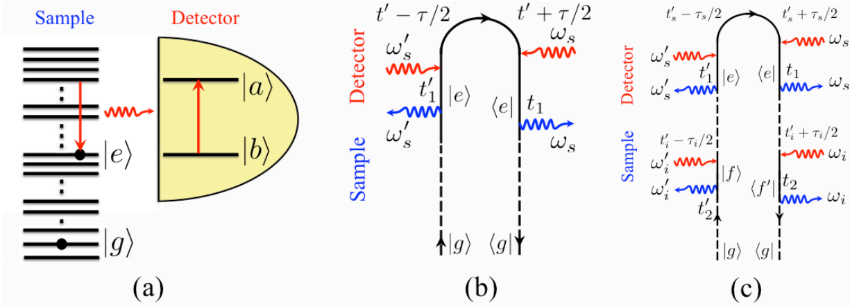
FIG. 21 (Color online) (a) Schematic of time-and-frequency resolved photon coincidence measurement. (b) Loop diagram for the bare signal (E15) in a gated measurement. (c) - Loop diagram for correlated two photons measurement (E26). Dashed lines represent the dynamics of the system driven by the field modes. \tau_i and \tau_s can be either positive or negative.
