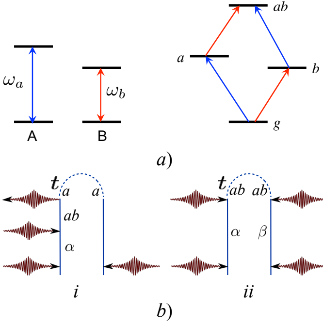
FIG. 6 (Color online) a) Scheme of two noninteracting two-level atoms A and B and corresponding many-body state diagram where ground state g corresponds to both atom in the ground state, a - atom A is excited and B is in the ground state, b - atom B is in the excited state and atom A is in the ground state, and ab - both atoms are in the excited state. Arrow directed upward represent two-photon excitation. b) Relevant set of diagrams corresponding to atom A being in excited state to \sim |\mu_A|^2 |\mu_B|^2 in field-matter interactions. \alpha, \beta run over a and b to account for all possible permutations in the excitation pathways.
