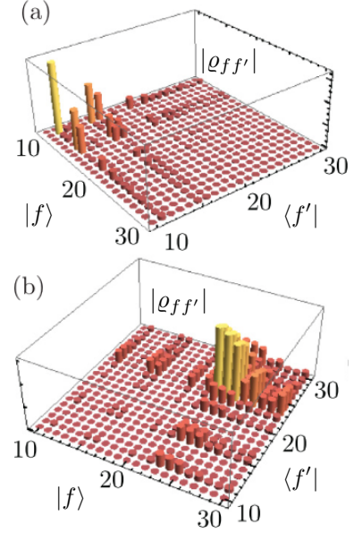
FIG. 9 a) The density matrix for doubly excited states \rho_{ff'}(t) = T_{f'g}^*(t)T_{fg}(t) , Eq. (100), prepared by the absorption of entangled photons with pump frequency \omega_p = 22,160 \text{ cm}^{-1} . b) the same, with \omega_p = 24,200 \text{ cm}^{-1} . [from (Schlawin et al. , 2012)]
