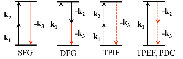
FIG. 27 Three wave process involuting classical (solid line) and quantum (dashed line) modes. Black lines represent incoming fields, red lines correspond to generated light.
