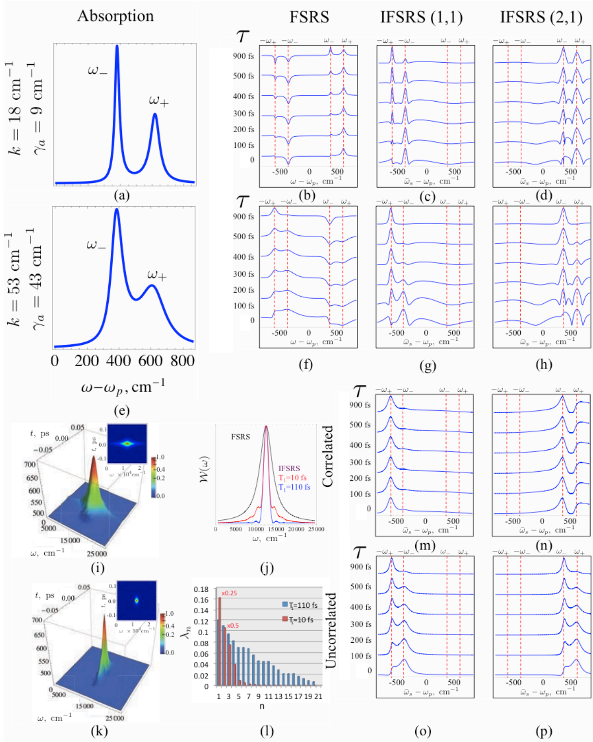
FIG. 26 (Color online) Top: (a) - Absorption, (b) - classical FSRS, (c) - S_{IFSRS}^{(1,1)} , (d) - S_{IFSRS}^{(2,1)} for a time evolving vibrational mode i vs \omega - \omega_p for slow tunneling rate and narrow dephasing, (e) - (h) are the same as (a) - (d) but for fast tunneling rate and broad dephasing. Bottom left: (i) - time-frequency Wigner spectrogram for classical light, (k) - same as (i) but for entangled twin state given by Eq. (204). Inserts depict a 2D projection. (j) - window function for FSRS \mathcal{E}_s^*(\omega)\mathcal{E}_s(\omega + i\gamma_a) -black, and IFSRS \Phi^*(\omega, \bar{\omega}_r)\Phi(\omega + i\gamma_a, \bar{\omega}_r) different values of T_1 . (l) - spectrum of the eigenvalues \lambda_n in the Schmidt decomposition (34) for entangled state with amplitude (205). Bottom right: S_{IFSRS}^{(1,1)} signal vs \bar{\omega}_s - \omega_p for correlated - (m) and uncorrelated - (o) separable states. (n), and (p) - same as (m) and (o) but for S_{IFSRS}^{(2,1)} signal. Parameters for simulations are listed in (Dorfman et al. , 2014).
