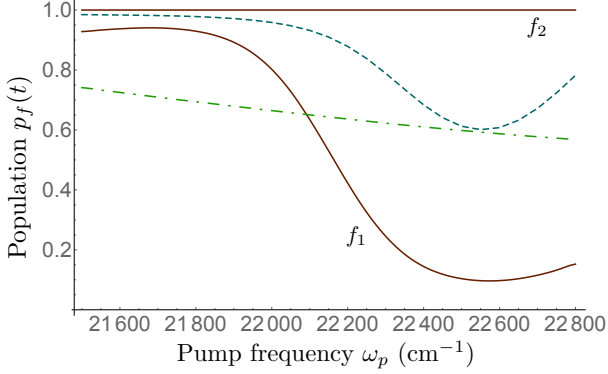
FIG. 10 Variation of the double-excited state populations p_f(t) , Eqs. (102)-(104) with the pump frequency \omega_p after excitation by entangled photons with strong frequency anti-correlations (solid, red), by laser pulses matching the pump bandwidth \sigma_p (blue, dashed), and laser pulses matching the photon bandwidths \sim 1/T (green, dot-dashed). The total f -population is normalized to unity at each frequency, i.e. \sum_f p_f(t) = 1 .
