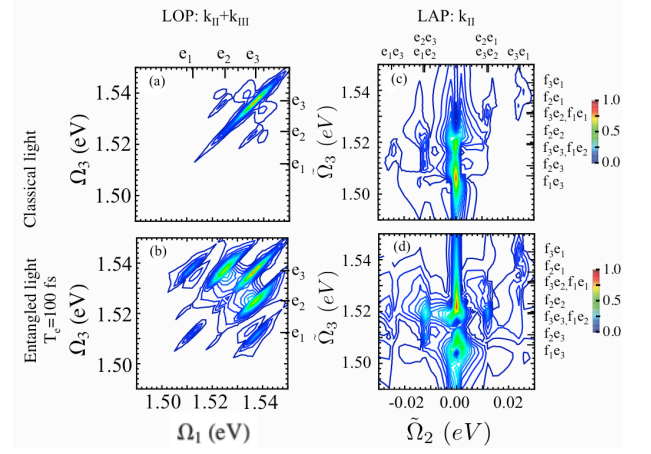
FIG. 18 (Color online) Left column: LOP signal S_{\mathbf{k}_{II}+\mathbf{k}_{III}}(\Omega_1, \tau_2 = 0, \Omega_3) for a molecular trimer with classical light Eq. (123) - (124) - (a), entangled light (125) with T_e = 100 fs - (b). Right: column: LAP signal S_{\mathbf{k}_{II}}(\tilde{\Omega}_1, t_2 = 0, \tilde{\Omega}_3) using classical light Eq. (119) - (c), entangled light with T_e = 100 fs, Eq. (128) - (d). Intraband dephasing \gamma_{ee'} = 1 meV. All other parameters are given in Section 5 of (Dorfman and Mukamel, 2014b).
