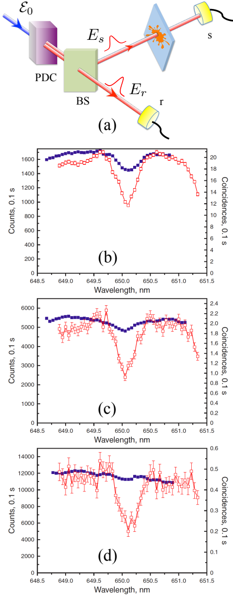
FIG. 22 (Color online) Linear absorption experiment of (Kalachev et al. , 2007) with coincidence detection. The entangled photon pair in beams E_s and E_r are split on a beam splitter. E_s is employed as a probe transmitted through the sample, while E_r is detected in coincidence - (a). The absorption spectrum of Er^{3+} ion in YAG crystal around 650 nm obtained by single photon counting (blue filled squares, left Y-axis) and coincidence counting (red open squares, right Y-axis) at various values of signal-to-noise ratio in the channel with the sample: 1/2 (b), 1/5 (c), and 1/30 (d)
