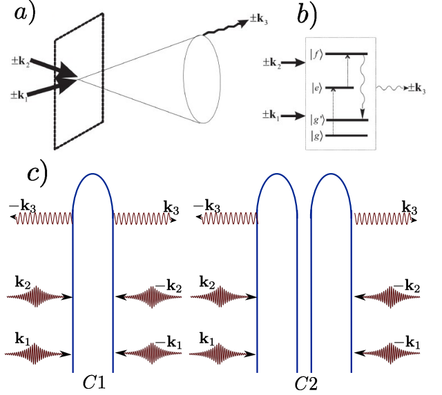
FIG. 30 Three wave process with two classical and one quantum mode: a) phase-matching condition; b) molecular level scheme; c) loop for the incoherent TPIF (C1) and coherent homodyne SFG (C2)
