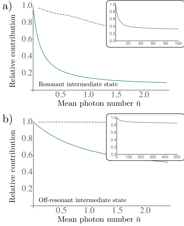
FIG. 11 a) Relative contribution of the coherent two-photon contribution h_{12} , Eq. (63), to the full time-integrated population of f_2 plotted vs. the mean photon number \bar{n} , Eq. (59). The dashed line shows strong entanglement with entanglement time T = 10 fs, and the solid line weaker entanglement with T = 100 fs. b) same for an intermediate state moved to \omega_{e_2} = 18,500 \text{ cm}^{-1} .
