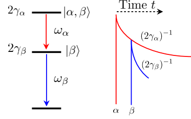
FIG. 7 (Color online) The temporal profiles of two photons emitted by a cascade source illustrate time-frequency entanglement: the red curve represents the marginal probability P(\tau_\alpha) Eq. (85), and the blue curve corresponds to the conditional probability P(\tau_\beta|\tau_\alpha) Eq. (84). The intrinsic time ordering of the photons, \alpha first, followed by \beta , suppress the excitation pathway where \beta is absorbed first, followed by \alpha , inducing joint two-atom excitation.
