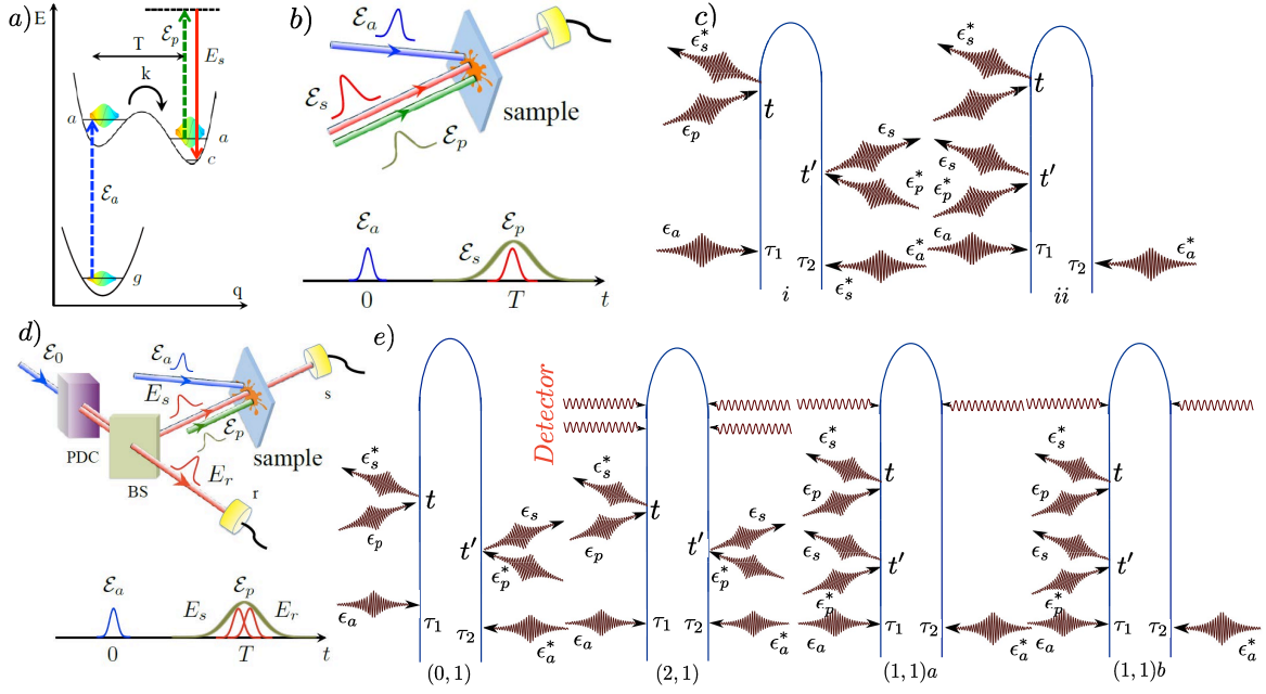
FIG. 25 (Color online) Top row: FSRs level scheme for the tunneling model - a , pulse configuration - b , loop diagrams (for diagram rules see Appendix A) - c . d and e - the same as b , and c but for FIFRS. The pairs of indices (0, 1) etc. indicate number of photons registered by detectors s and r in each photon counting signal: (N_s, N_r)
