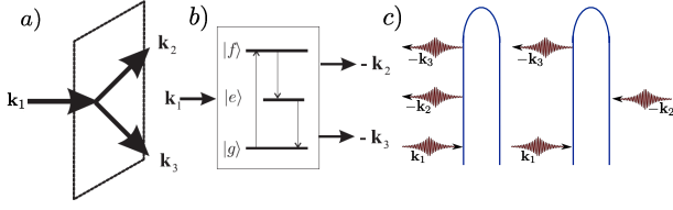
FIG. 28 Heterodyne detected DFG: (A) phase matching condition \mathbf{k}_3 = \mathbf{k}_1 - \mathbf{k}_2 ; (B) molecular level scheme; (C) loop diagrams.
