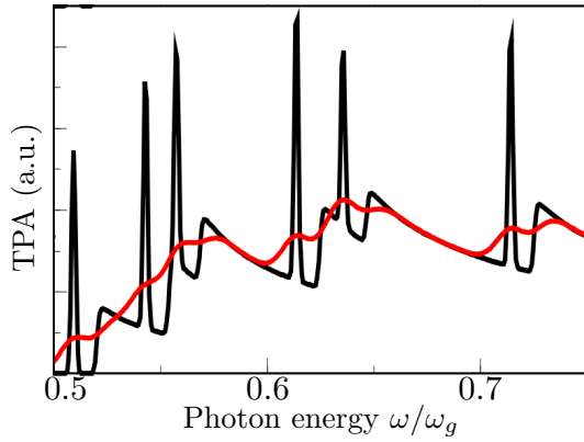
FIG. 14 Two-photon absorption (TPIF in our notation, see section. III.B.1) in a semiconductor quantum well [taken from (Salazar et al. , 2012)]: excited state resonances within a continuum of delocalized states may be enhanced with frequency anti-correlations (black) or suppressed with positive frequency correlations (red).
