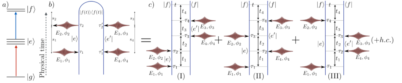
FIG. 2 Diagrammatic construction of the double excitation probability \rho_{ff} in a three level model a). b) The single loop diagram representing the evolution of the wavefunction. On the left hand side, the vertical line represents ket and the right hand it corresponds to the bra. The wave function in this closed time path loop diagram propagates forward in a loop from the bottom branch of the diagram along the ket branch to the top of the diagram. It then evolves backward in time from the top to the bottom of the right branch (bra). This forward and backward propagation is similar to the Keldysh contour diagram rules (Keldysh, 1965). Horizontal arrows represent field-matter interactions. c) The corresponding three ladder diagrams for the evolution of the density matrix. Here the density matrix evolves forward in time upward from the bottom to the top of the diagram. In order to achieve doubly excited state population starting from the ground state the density matrix has to undergo four interactions represented by the absorption of two photons represented by four inwardly directed arrows. The three diagrams represent different time orderings of ket vs bra interactions. These are lumped together in the single loop diagram b)
