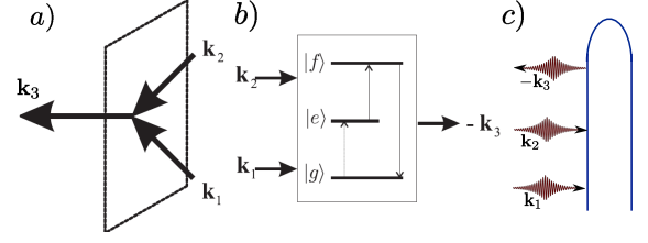
FIG. 29 Heterodyne detected SFG: (A) phase matching condition \mathbf{k}_3 = \mathbf{k}_1 + \mathbf{k}_2 ; (B) level scheme; (C) loop diagrams.
