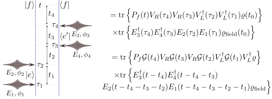
FIG. 39 Ladder diagram construction in a QED formulation: Using the diagram rules given in the text, the diagram translates into the Heisenberg picture expression (top) or the Schrödinger picture expression (bottom). The corresponding field correlation functions are reordered as in the loop diagram.
