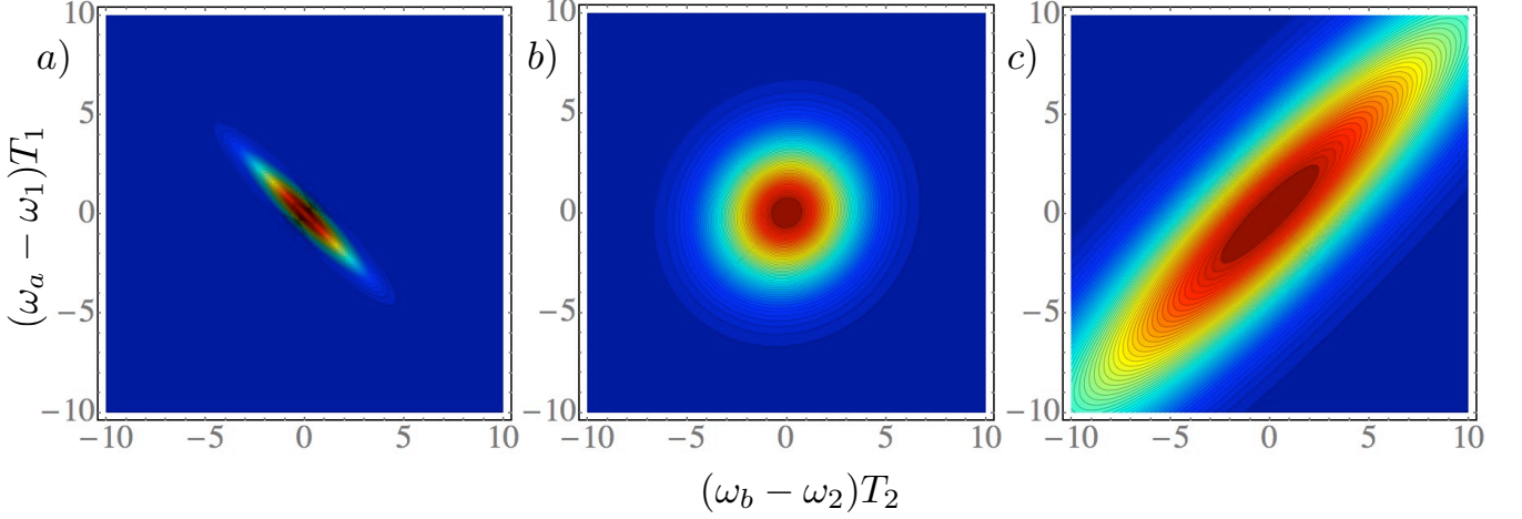
FIG. 3 Absolute value of the two-photon correlation function (63) of entangled photon pairs with a) strong frequency anti-correlations, \sigma_p = 0.6 / T_2 [entanglement entropy (40) E = 1.9 ], b) very weak correlations ( E = 0.018 ), \sigma_p = 3.5 / T_2 , and c) strong positive frequency correlations, \sigma_p = 50 / T_2 ( E = 1.7 ).
