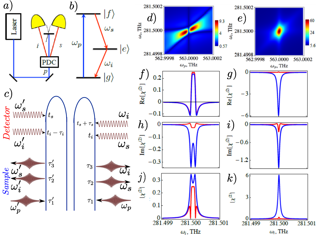
FIG. 33 (Color online) Left: Schematic of the PDC experiment - (a), the three level model system used in our simulations - (b). One out of four loop diagram (remaining three diagrams are presented in Ref.(Dorfman and Mukamel, 2012b)) for the PCC rate of signal and idler photons generated in type I PDC (Eq. (265)) - (c). The left and right diagrams represent a pair of molecules. Blue (red) arrows represent field-matter interaction with the sample (detectors). There are four possible permutations ( s/i and s'/i' ) which leads to four terms when Eq. (267) is substituted into Eq. (266). Right: Absolute value of semiclassical susceptibility |\chi_{+-}^{(2)}(-(\omega_p - \omega_i), -\omega_i, \omega_p)| (arb. units) (268) - (d), and quantum the susceptibility |\chi_{LL-}^{(2)}(-(\omega_p - \omega_i), -\omega_i, \omega_p)| (267) - (e) vs pump \omega_p and idler frequency \omega_i . We used the standard KTP parameters outlined in the text. Left column: real - (f), imaginary part - (h) and absolute value - (j) of \chi_{+-}^{(2)} - red line and \chi_{LL-}^{(2)} - blue line for off resonant pump \omega_p - \omega_{gf} = 10\gamma_{gf} . Right column: (g,i,k) - same as (f,h,j) but for resonant pump \omega_p \simeq \omega_{gf} .
