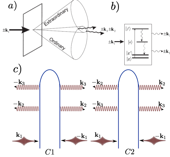
FIG. 32 Type II PDC: (A) phase matching, (B) molecular level scheme; (C) CTPL diagrams for the signal from k_3 (C1) and k_2 (C2) modes polarized along x direction.
