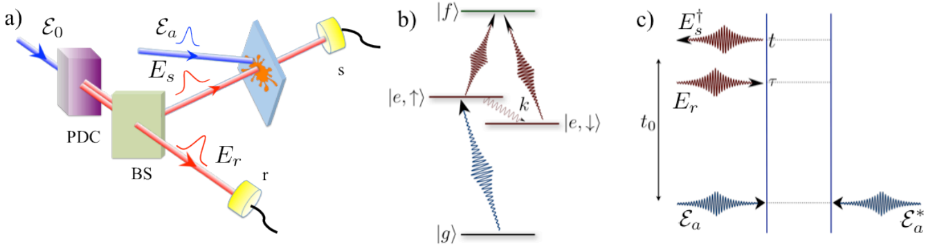
FIG. 23 (Color online) a) The IPP setup: the entangled photon pair in beams E_s and E_r are split on a beam splitter. A classical, actinic, ultrafast pulse \mathcal{E}_a excites the sample, and E_s is employed as a probe in a pump-probe measurement, while E_r is detected in coincidence. b) The level scheme for the two-state jump (TSJ) model considered in this work. The g - e transition is far off-resonant from the spectral range of the entangled photon wavepacket, which only couples to the e - f transition. c) Diagram representing the pump-probe measurement. [taken from (Schlawin et al. , 2015)]
