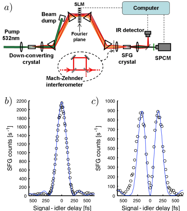
FIG. 5 (Color online) a) Experimental layout of the entangled photon shaper: A computer-controlled spatial light modulator (SLM) is used to manipulate the spectral phase of the entangled photons. The photon pairs are detected in the inverse process of PDC - sum frequency generation (SFG). The SFG photons are subsequently counted in a single-photon counting module. In order to demonstrate two-photon interference oscillations, a Mach-Zehnder interferometer is placed between the last prism and the SFG crystal. b) The SFG counts (circles) and the calculated second-order correlation function (line) of the unperturbed wavefunction as a function of the signal-idler delay. c) the same for the shaped wavefunction. Figure is taken from (Pe'er et al. , 2005).
