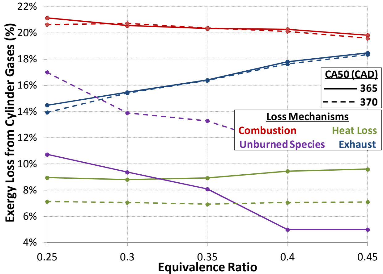
Figure 13 - Equivalence ratio sweep of exergy loss mechanisms for P_{BDC}=1.8 bar abs, 1800 RPM, CA50=365° and 370°, Ethanol fuel
