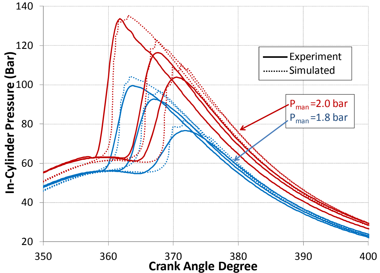
Figure 1 - Comparison of experimental and simulated in-cylinder pressure traces
