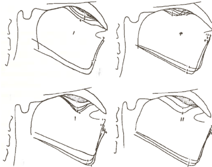
Figure 4.4: Differences in tongue movements in production of |, †, !, ||
