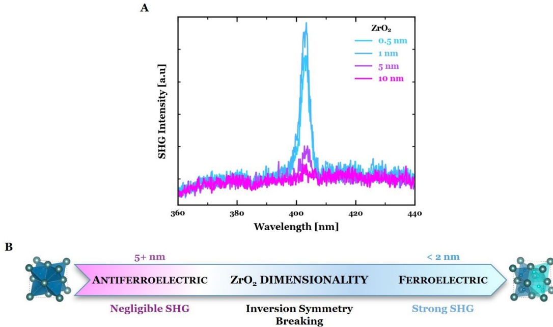
Fig. S11. Second harmonic generation (SHG) spectra. (A) SHG spectrum for ultrathin (0.5 nm, 1 nm) ferroelectric \text{ZrO}_2 films and relatively thick (5 nm, 10 nm) antiferroelectric \text{ZrO}_2 films, which demonstrate strong and negligible SHG intensity around 405 nm (810 nm fundamental laser beam), respectively, consistent with the SHG mapping trends (Fig. 2C). (B) Dimensionality-driven evolution of \text{ZrO}_2 from the nonpolar antiferroelectric phase to the polar ferroelectric phase indicated by inversion symmetry breaking.
