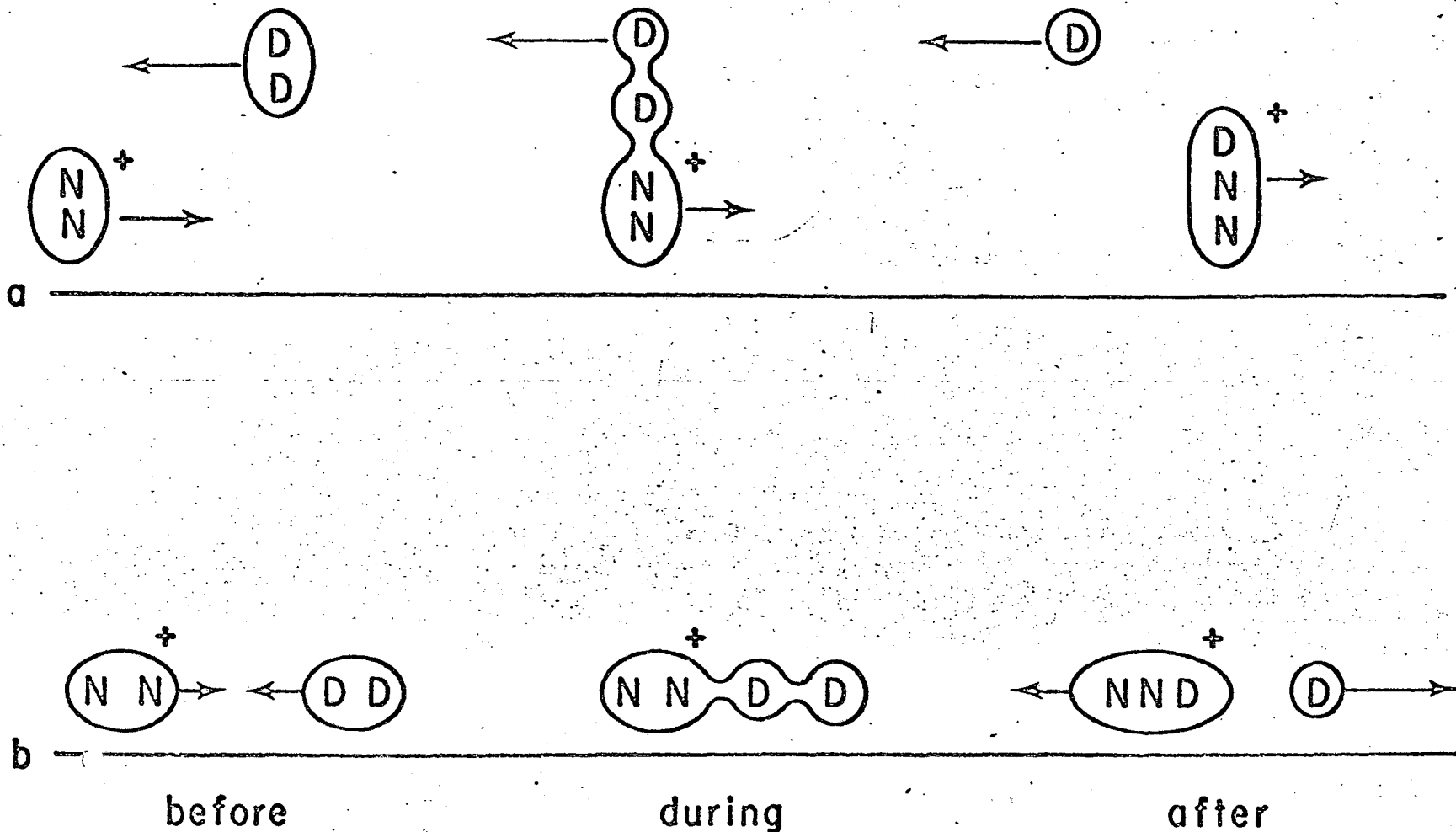
Figure 5. Schematic representation of reactive collisions.
