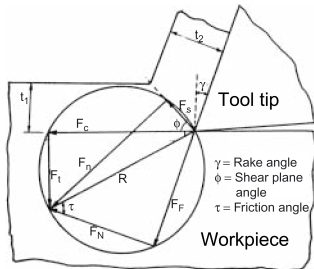
Fig. 3.1 Forces at work in chip cutting [25]
