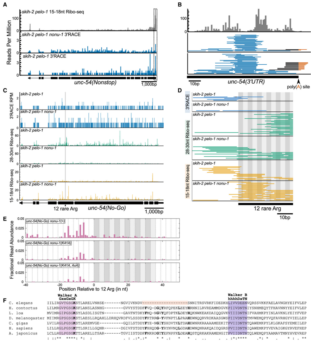
Figure 4. nonu-1-Dependent mRNA Cleavage Occurs in the Vicinity of Stalled Ribosomes
