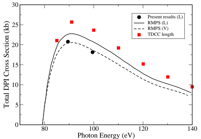
FIG. 1: (Color online) Total DPI cross section of lithium from the 1s^2 2p, ^2P excited state. RMPS and TDCC results from ref. [8]. 1 \text{ kb} = 10^{-21} \text{ cm}^2 .
