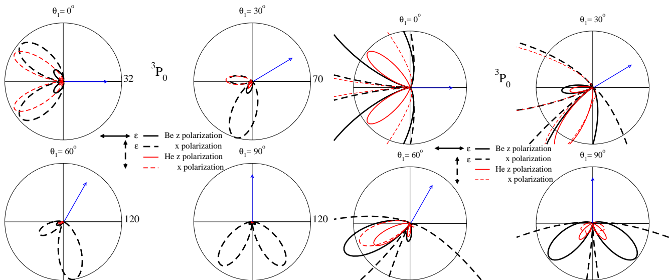
FIG. 7: (Color online) As in Fig. 6, for ^3P_0 beryllium and ^3P_0 helium.
