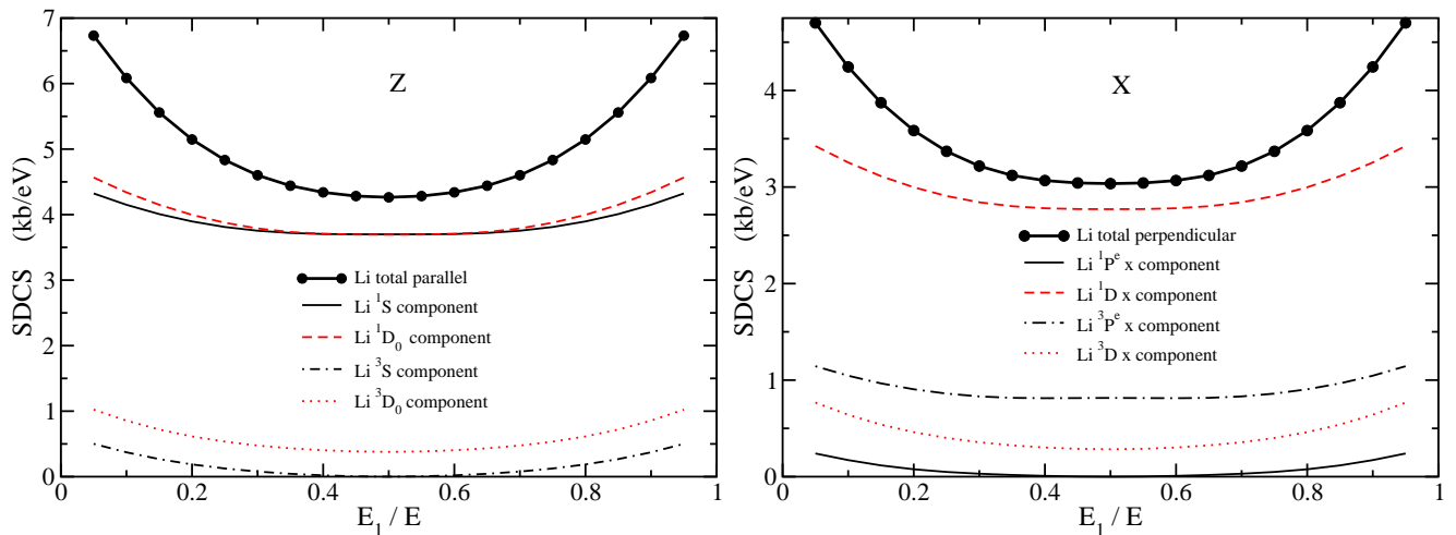
FIG. 5: (Color online) Singly differential cross sections for double ionization of {}^2P_0 lithium at 10 eV above threshold. Singlet (solid curves) and triplet (dashed curves) contributions are individually labelled. Left panel: z-polarization; right panel: x-polarization.
