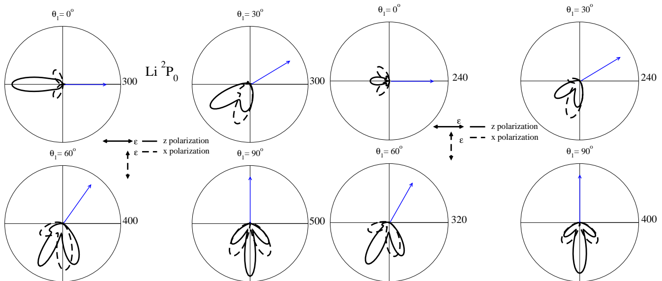
FIG. 8: (Color online) Four left panels: triply differential cross sections for double ionization of ^2P_0 lithium with z- and x-polarized light at 10 eV above threshold and equal energy sharing. The four right panels show TDCS using beryllium data, but combined as in they would be for lithium (see text). Radii of circles, marked to the right, give magnitude of cross sections in units of b/eV/sr^2 .
