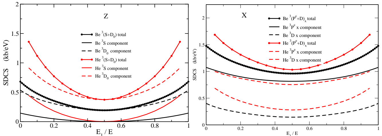
FIG. 4: (Color online) As in Fig. 3, for ^3P_0 beryllium and ^3P_0 helium.
