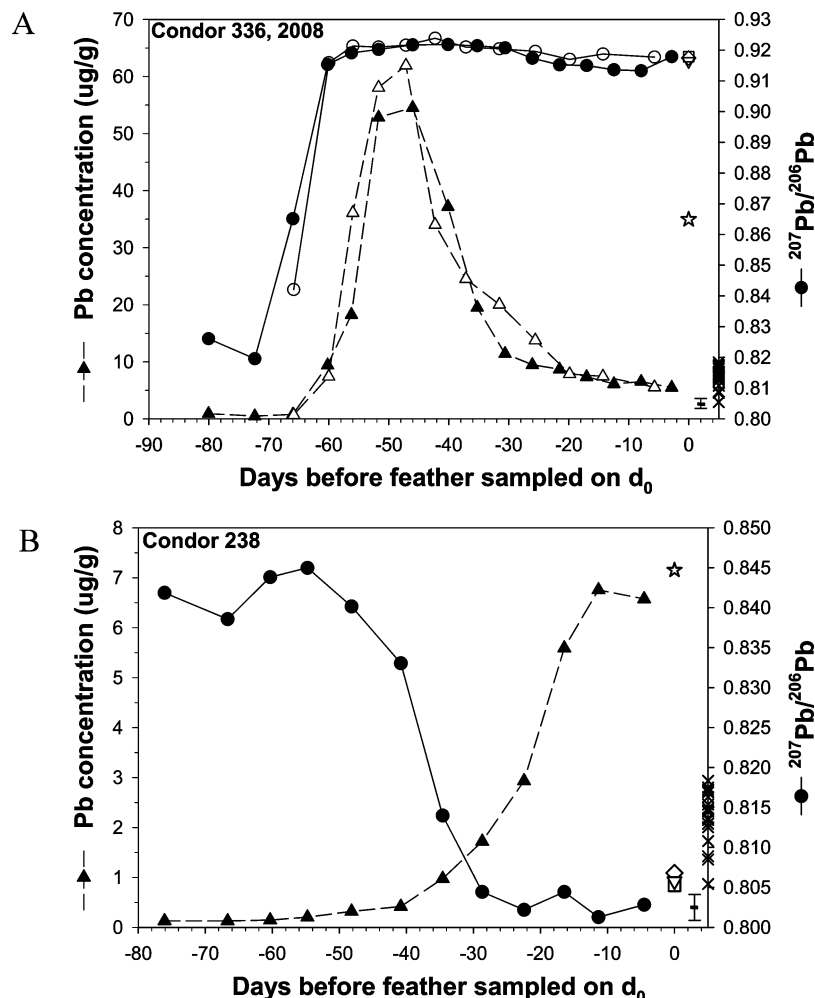
FIGURE 2. (A) Segments from condor 336 primary feather ^{207}\text{Pb}/^{206}\text{Pb} ratios ( \bullet ) and lead concentrations ( \blacktriangle ) and retrix feather ^{207}\text{Pb}/^{206}\text{Pb} ratios ( \circ ) and lead concentrations ( \triangle ) versus days before d_0 , the date the feathers were sampled (immediately following death). Lead ammunition from California reported by Church et al. (4) is represented by \times (along the right y-axis). ^{207}\text{Pb}/^{206}\text{Pb} ratios in blood ( \nabla ), kidney ( \diamond ), and liver ( \square ) collected pre- and postmortem (plotting on top of one another in the upper right) are identical and match the ^{207}\text{Pb}/^{206}\text{Pb} ratios in feather vane grown after exposure ( \sim d_{-70} ). The ^{207}\text{Pb}/^{206}\text{Pb} ratios in bone ( \star ) were intermediate between the ^{207}\text{Pb}/^{206}\text{Pb} ratios of the blood and soft tissues and most distal (pre-exposure, oldest) feather segment. The ICP-MS measurement error is shown in the lower right ( - ) \pm 2 SD. (B) Condor 238 feather ^{207}\text{Pb}/^{206}\text{Pb} ratios ( \bullet ) and lead concentrations ( \blacktriangle ) in primary feather segments versus days before d_0 , the date the feather was sampled (immediately following death). The ^{207}\text{Pb}/^{206}\text{Pb} signature falls within the range of lead ammunition from California ( \times , along the right y-axis) reported by Church et al. (4). ^{207}\text{Pb}/^{206}\text{Pb} ratios in blood ( \nabla ), kidney ( \diamond ), and liver ( \square ) collected pre- and postmortem (plotting on top of one another in lower right) are identical and match the ^{207}\text{Pb}/^{206}\text{Pb} ratios in the feather vane grown after exposure ( \sim d_{-50} ), while the bone ^{207}\text{Pb}/^{206}\text{Pb} ratio ( \star ) is consistent with values observed in the pre-exposure (oldest) feather segments. The ICP-MS measurement error is shown in the lower right ( - ) \pm 2 SD.
